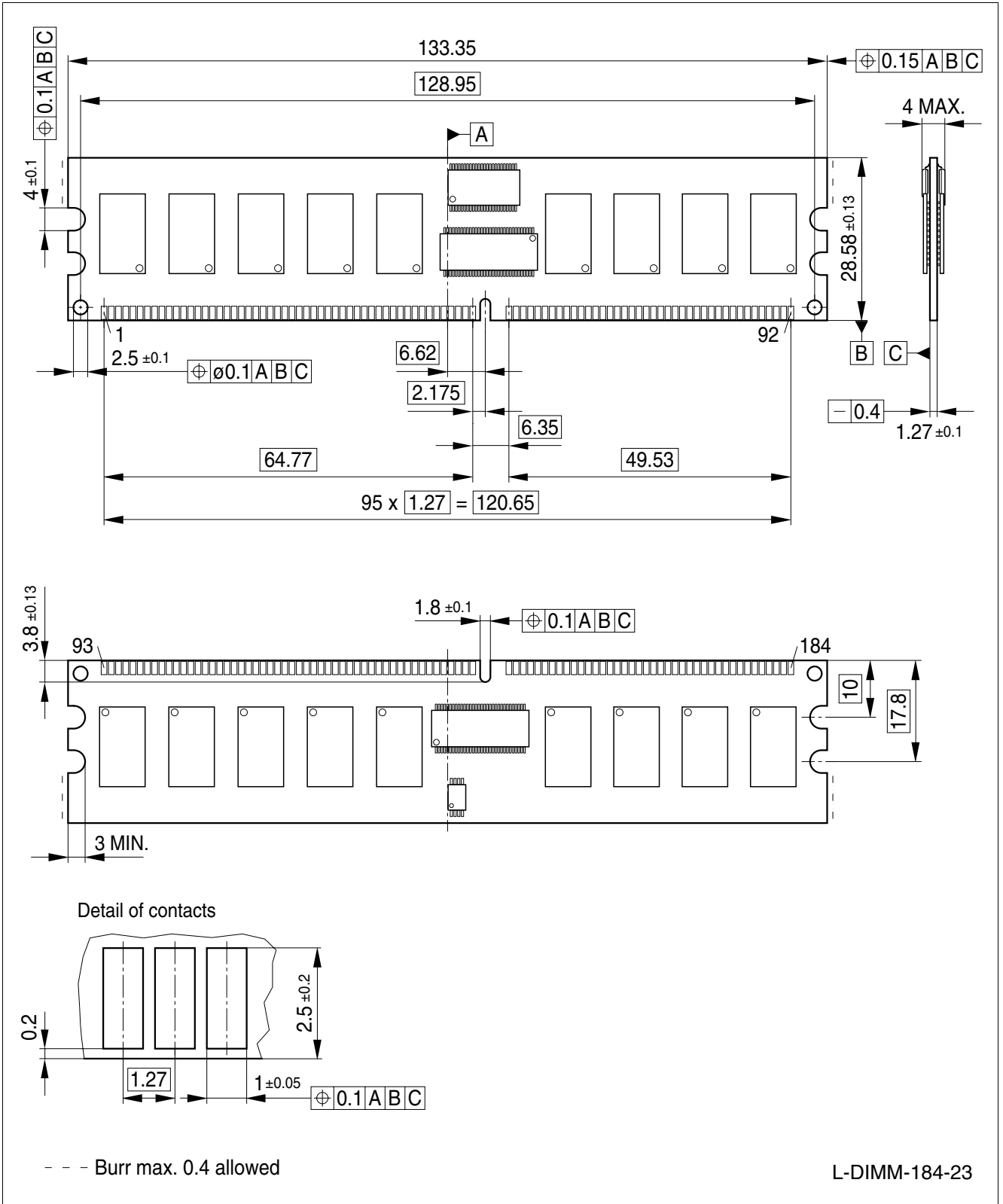
Figure 8 Package Outlines – Raw Card B HYS72D64320GBR-[5/6]-C (2 Ranks \times 8)
