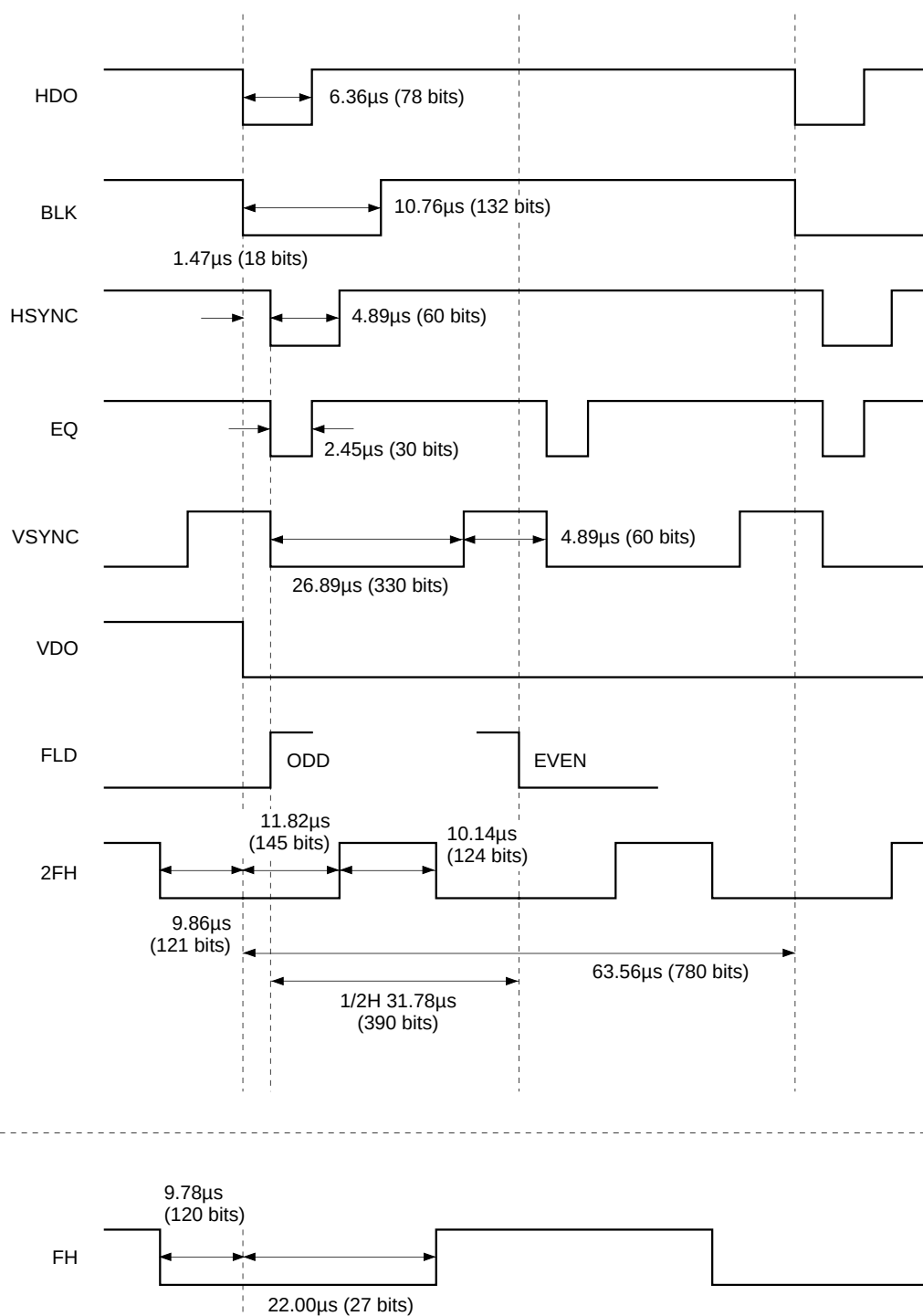
Timing Chart (9) &lt;SG horizontal direction&gt;
