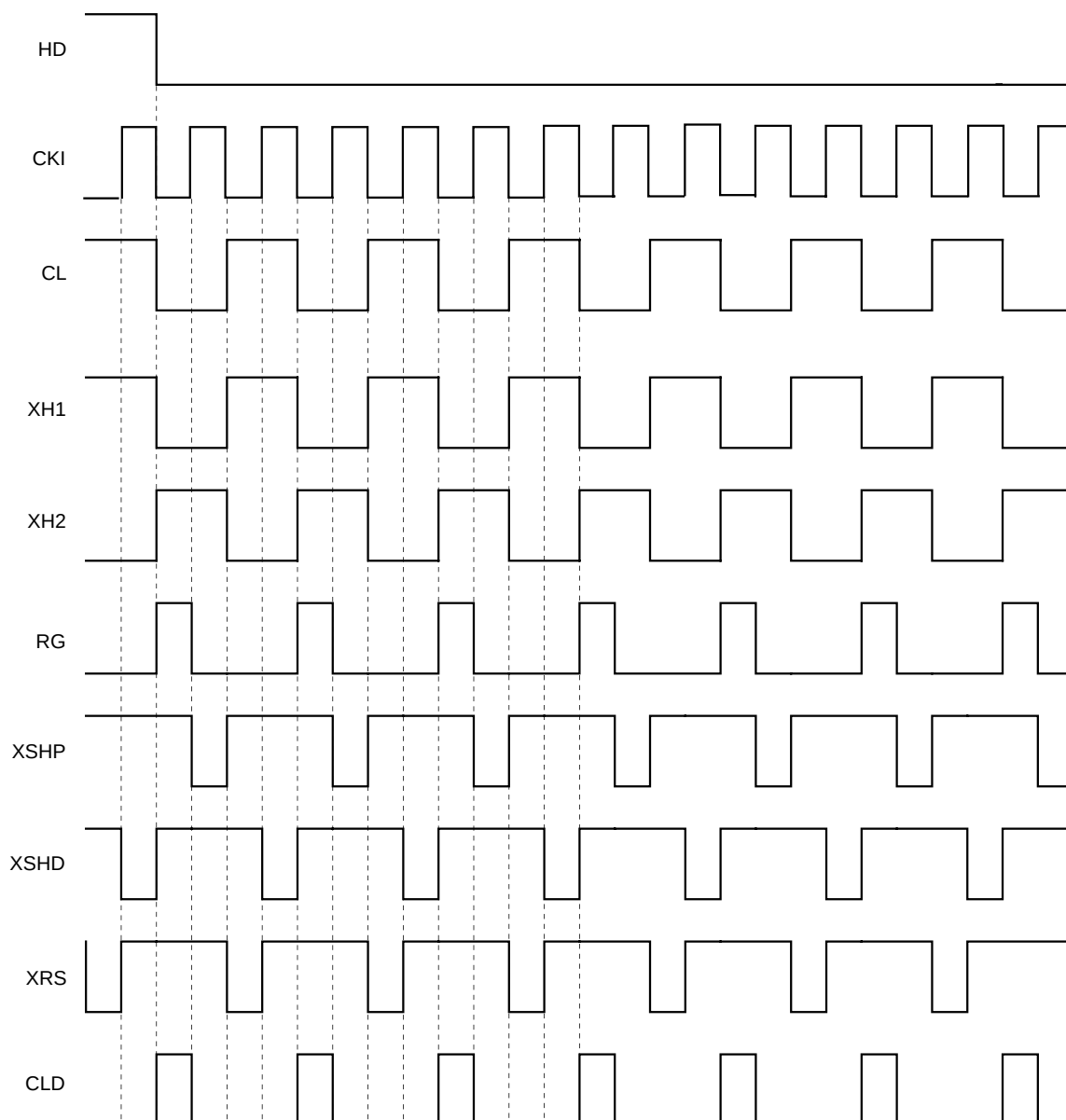
Timing Chart (7) &lt;High-speed phase&gt;
