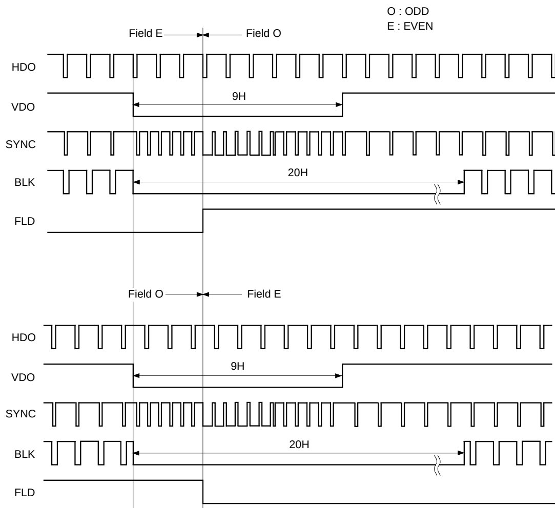
Timing Chart (8) &lt;SG vertical direction&gt;
