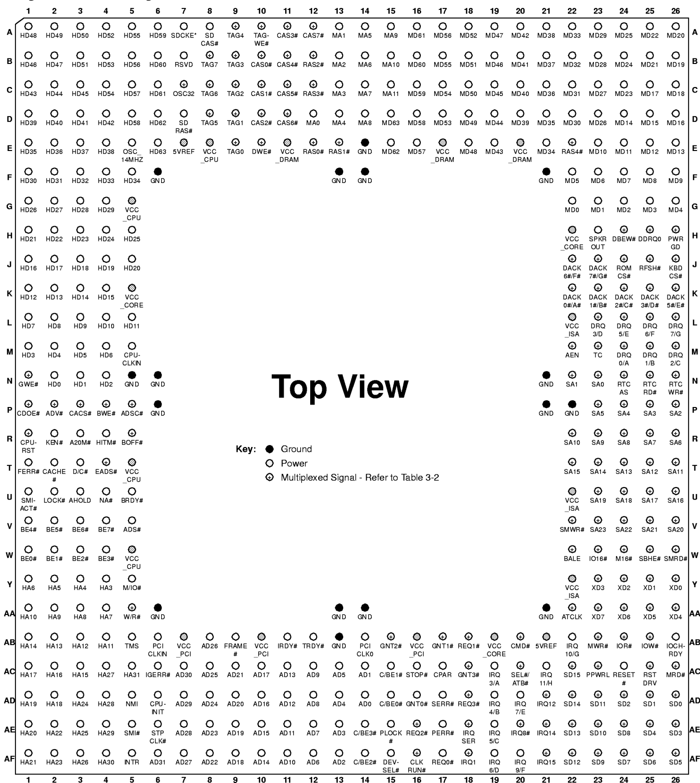
Figure 3-1 Pin Diagram
