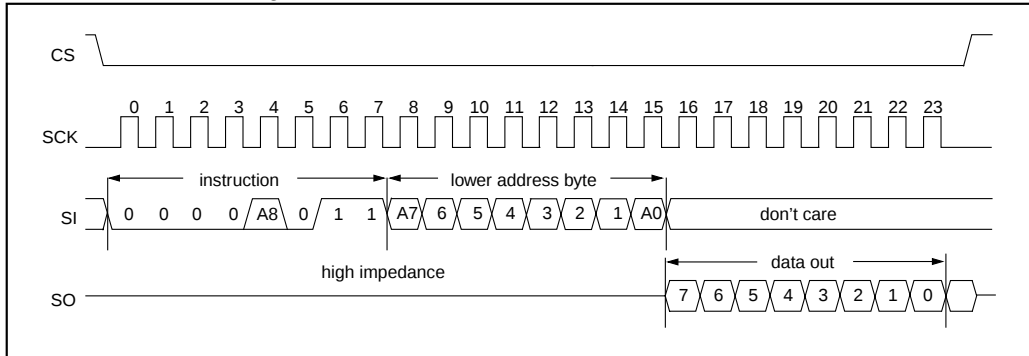
FIGURE 3-3: BYTE WRITE SEQUENCE
