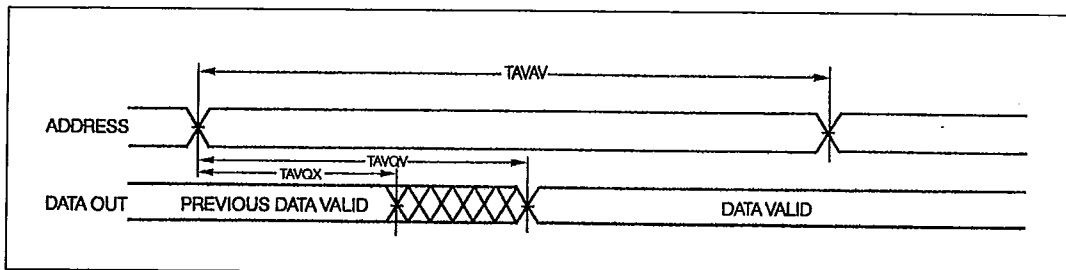
READ CYCLE nb 1
