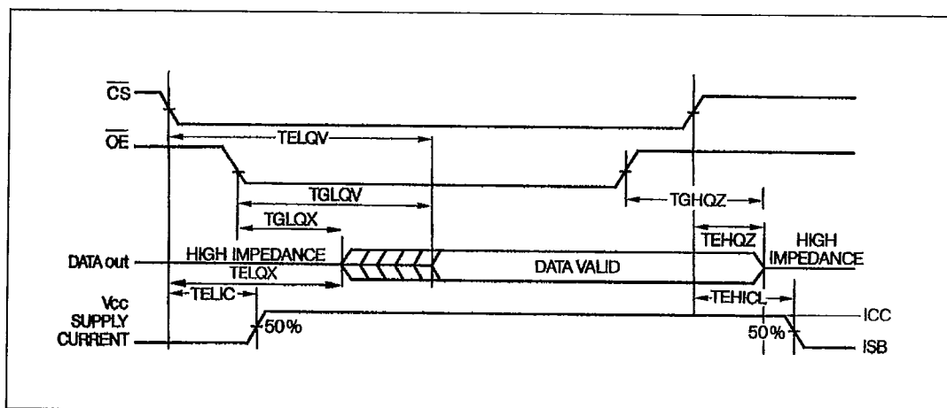
READ CYCLE nb 2
