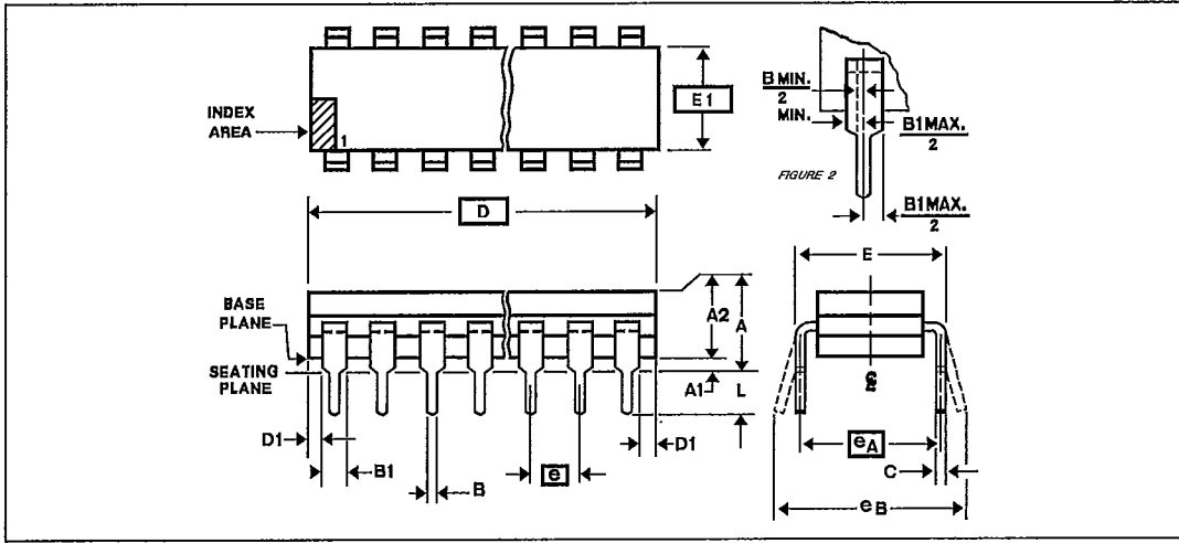
28 PINS CERDIP .300
