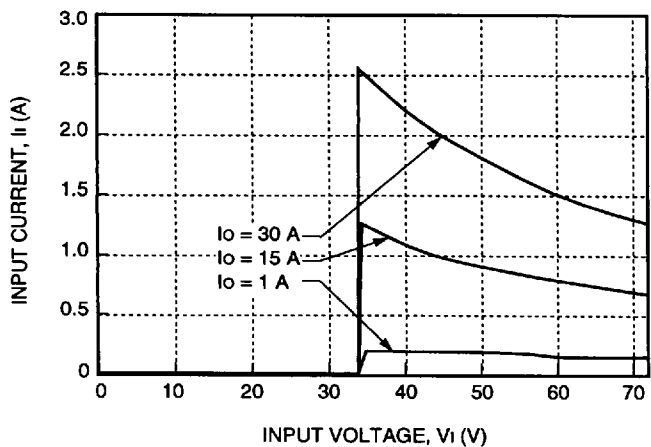
Figure 1. Typical FW150D Input Characteristics at Room Temperature
