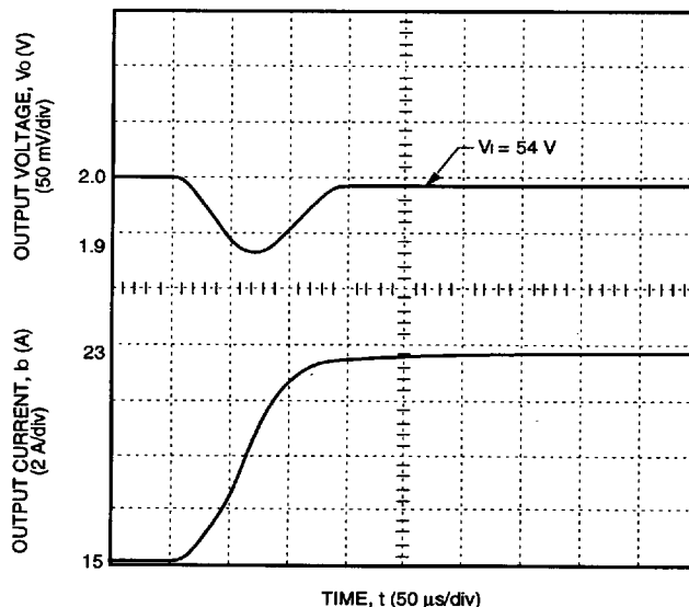
Figure 7. Typical FW150D Transient Response to Step Increase in Load from 50% to 75% of Full Load at Room Temperature (Waveform Averaged to Eliminate Ripple Component.)
