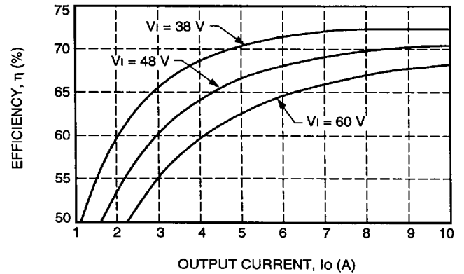
Figure 3. Typical FE050D Efficiency vs. Output Current at Room Temperature
