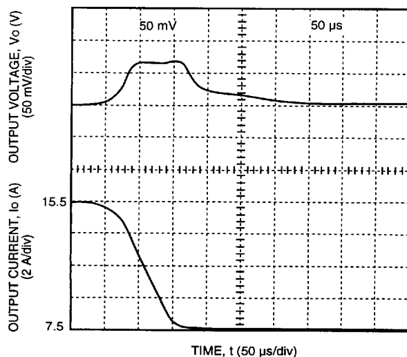
Figure 6. Typical FE150D Transient Response to Step Decrease in Load from 50% to 25% of Full Load at Room Temperature and 48 V Input (Waveform Averaged to Eliminate Ripple Component.)
