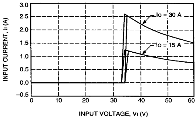
Figure 1. Typical FE150D Input Characteristics at Room Temperature
