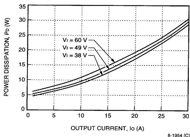
Figure 22. Power Dissipation vs. Output Current
