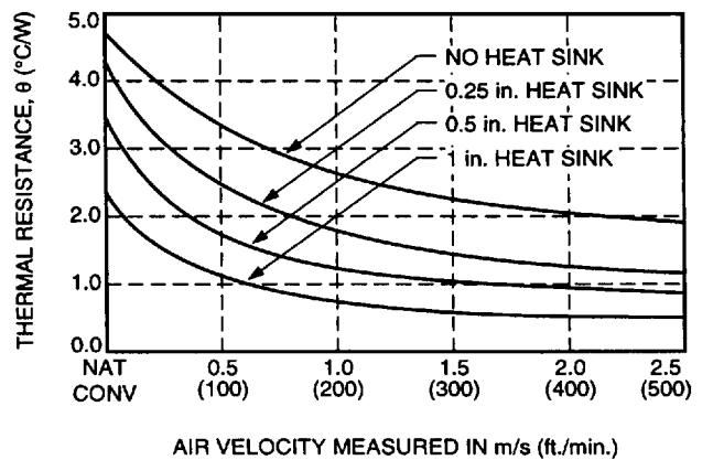
Figure 21. Heat Sink Resistance Curves; Fins Oriented Along Length
