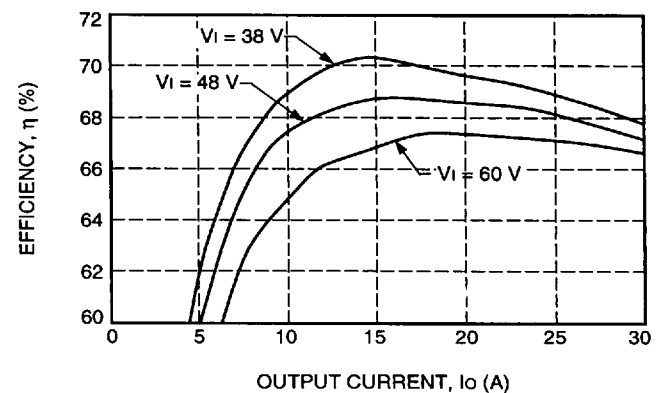
Figure 4. Typical FE150D Efficiency vs. Output Current at Room Temperature
