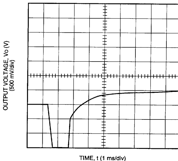
Figure 8. Typical FE150D Start-Up Transient at Room Temperature, 48 V Input, and 30 A Output
