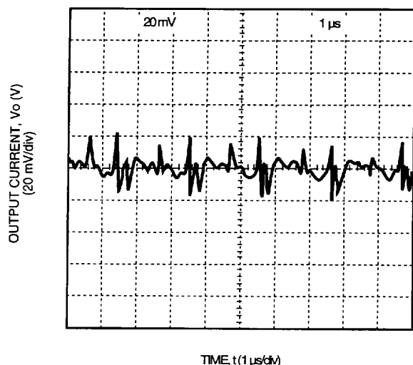
Figure 5. Typical FE150D Output Ripple Voltage at Room Temperature, 48 V Input, and 30 A Output
