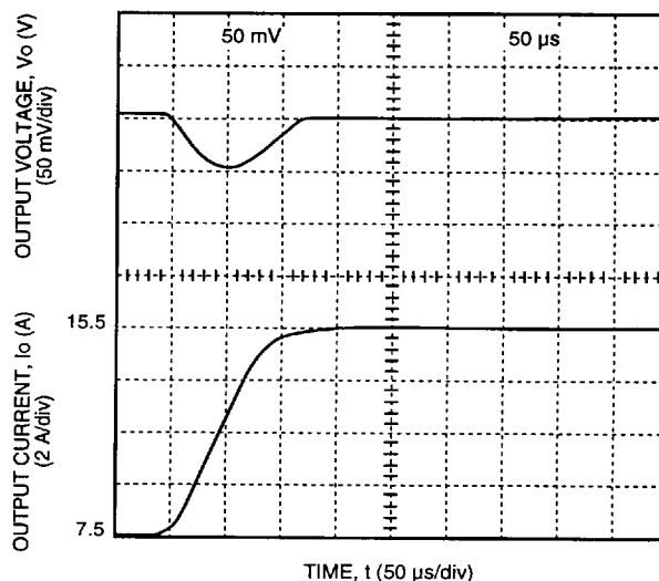
Figure 7. Typical FE150D Transient Response to Step Increase in Load from 50% to 75% of Full Load at Room Temperature and 48 V Input (Waveform Averaged to Eliminate Ripple Component.)
