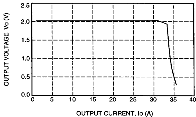
Figure 2. Typical FE150D Output Characteristics at Room Temperature and 48 V Input
