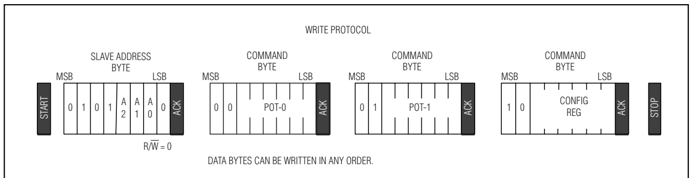
Figure 2. Write Protocol
