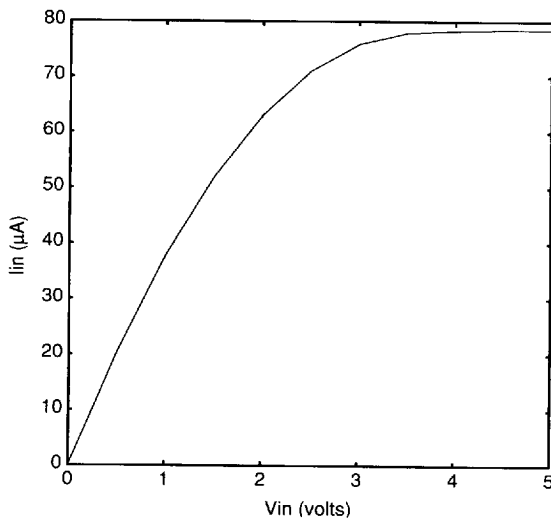
N-Channel Pull-Down Device
