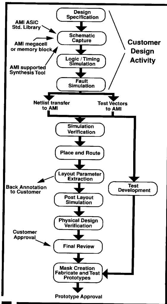
FIGURE 3: ASIC DESIGN FLOW
