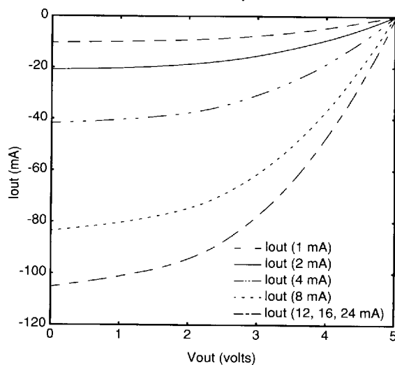
P-Channel Output Driver
