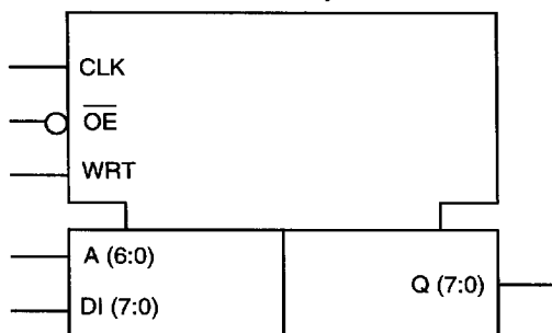
FIGURE 1: LOGIC SYMBOL
