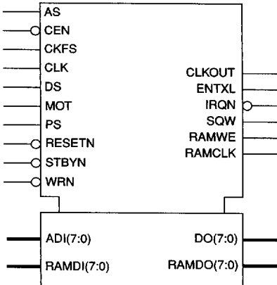
LOGIC SYMBOL MG1468C18
