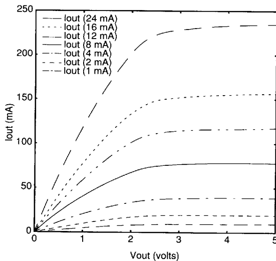
N-Channel Output Driver
