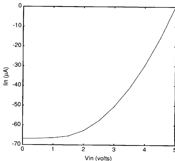
P-Channel Pull-Up Device
