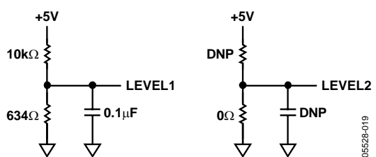
Figure 17. Flexible Circuits to Set the LEVEL1 and LEVEL2 Inputs to Obtain a 600 mV Output Offset on a Single Supply
