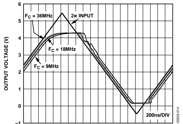
Figure 14. Overdrive Recovery vs. Cutoff Frequency
