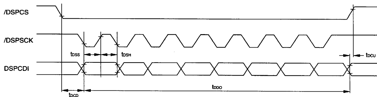
Fig. 10 DSP Interface Timing
