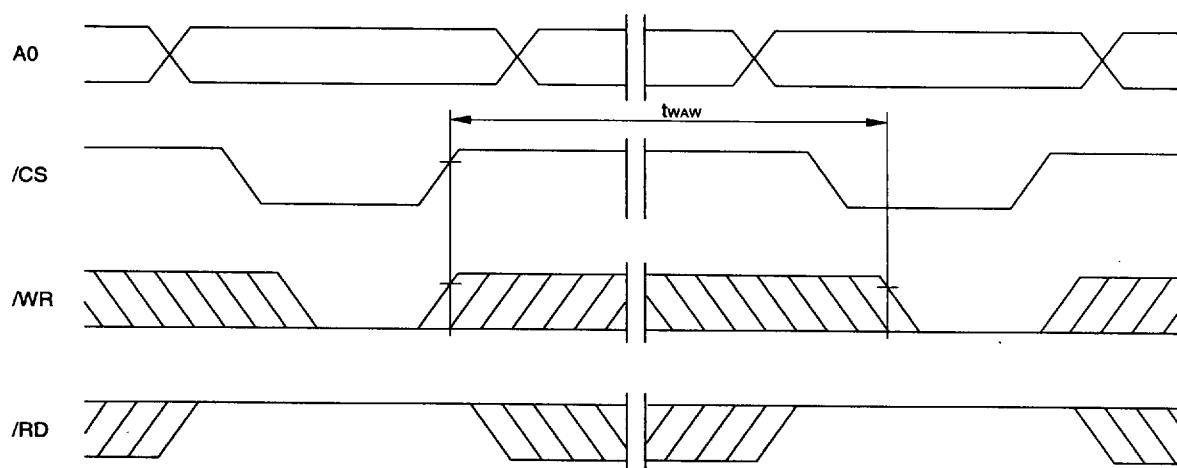
Fig. 6 CPU Interface Timing ④
