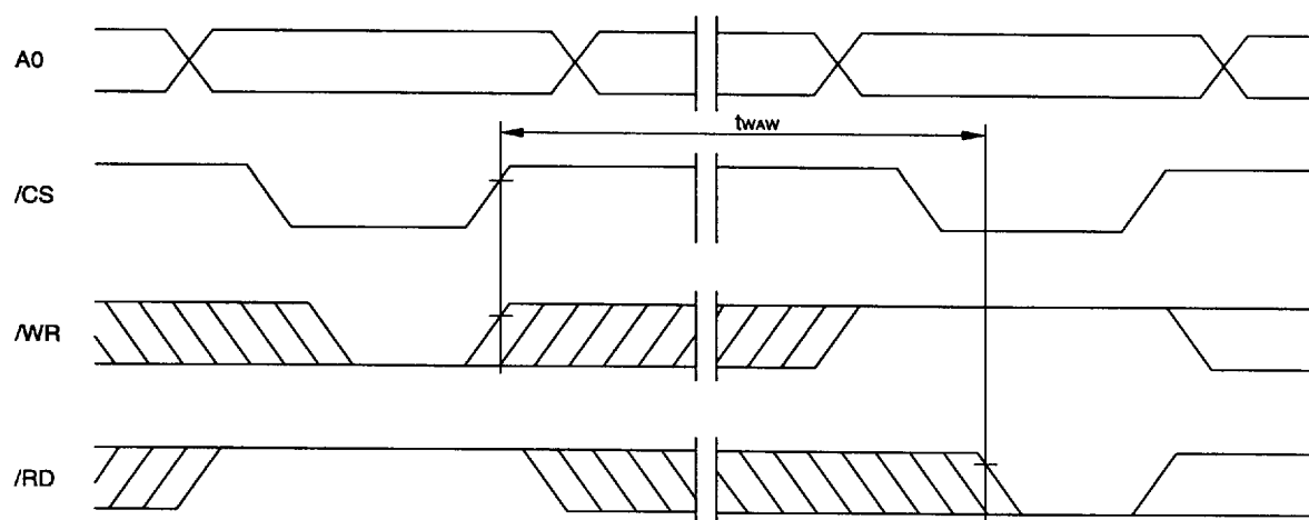
Fig. 5 CPU Interface Timing ③
