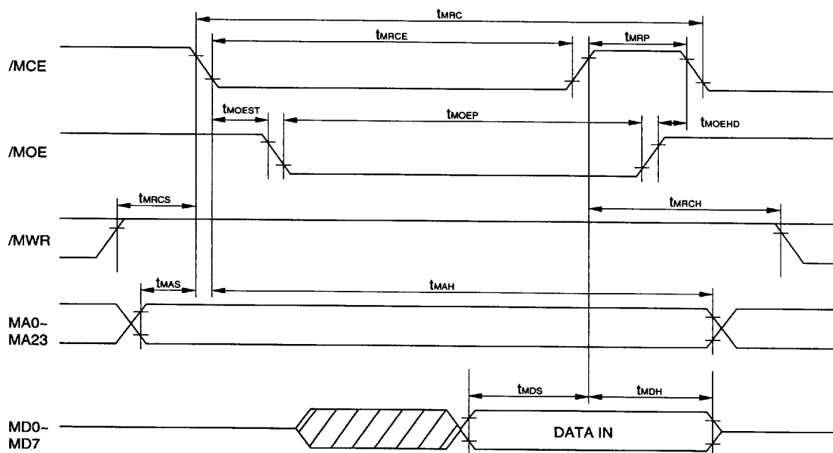
Fig. 8 External Memory Read Timing
