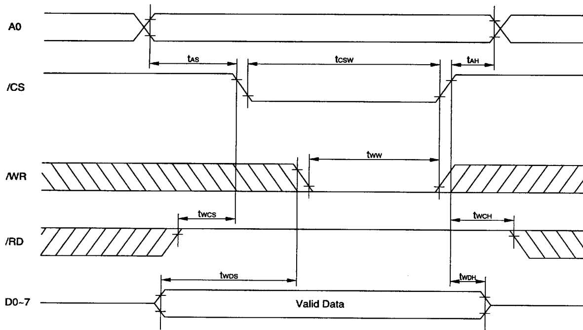
Fig. 3 CPU Interface Timing ①
