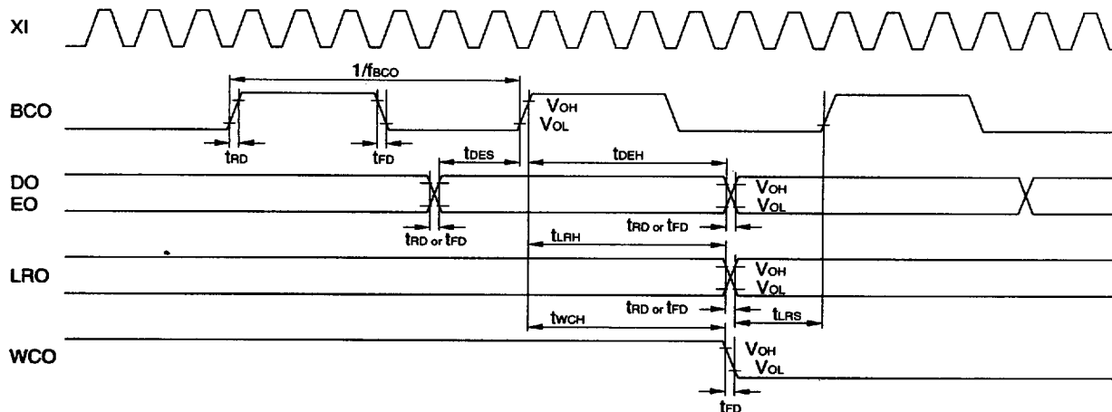
Fig. 9 Voice Data Output Timing
