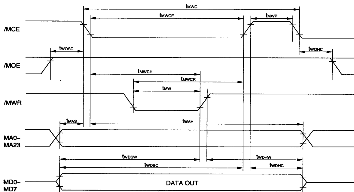
Fig. 7 External Memory Write Timing
