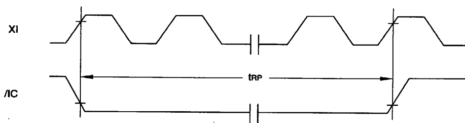
Fig. 2 Reset Timing
