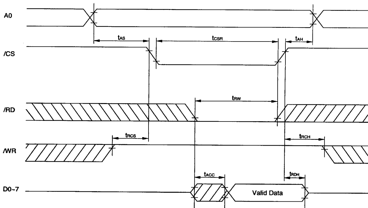
Fig. 4 CPU Interface Timing ②
