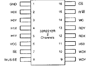
16-Lead SOL
