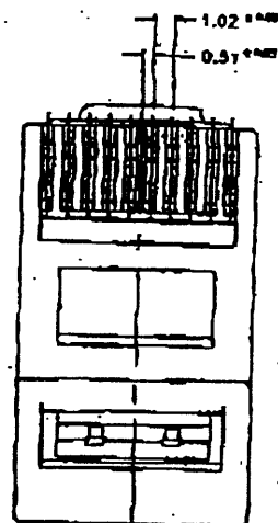
#112: MP10P10C-R
