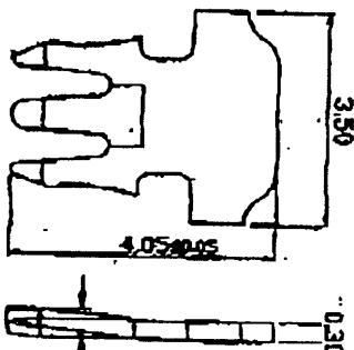
"3": 3 PRONGS FOR SOLID WIRE(S) 單芯線用三叉型金片
