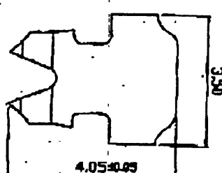
"2": 2 PRONGS FOR SOLID WIRE(S) 單芯線用大插角型金片
