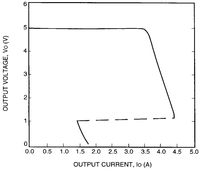
Figure 5. MW010A Typical Output Characteristic; V_i = 48\text{ V} ; T_A = 25\text{ }^\circ\text{C}
