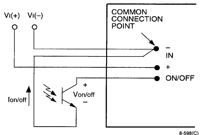
Figure 23. Remote On/Off Wiring Configuration
