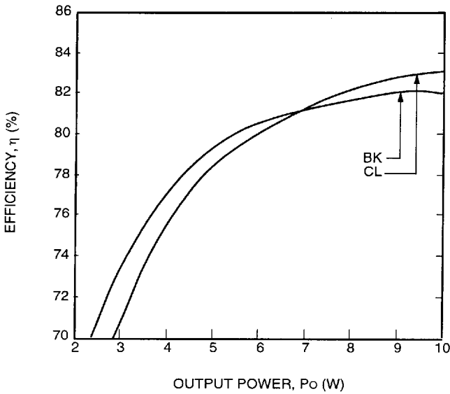
Figure 9. MW010BK, CL Typical Converter Efficiency as a Function of Output Power; V_i = 48\text{ V} ; T_A = 25\text{ }^\circ\text{C}
