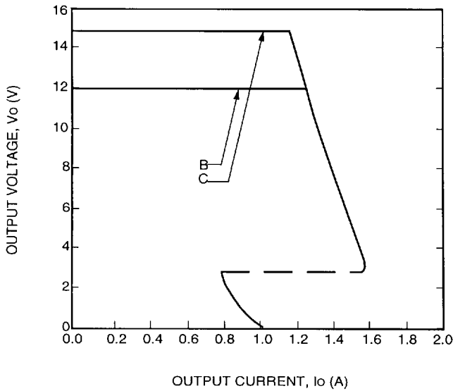
Figure 6. MW010B, C Typical Output Characteristic; V_i = 48\text{ V} ; T_A = 25\text{ }^\circ\text{C}
