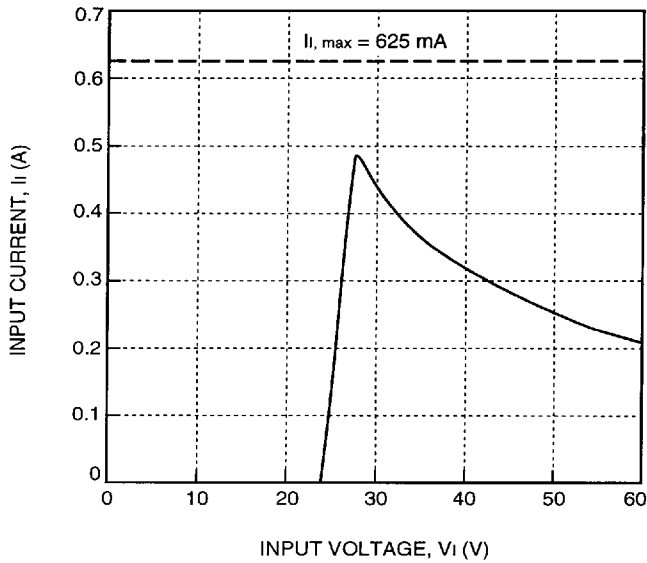
Figure 1. Typical Input Characteristic; I_o = I_{o, max} ; T_A = 25^\circ\text{C}
