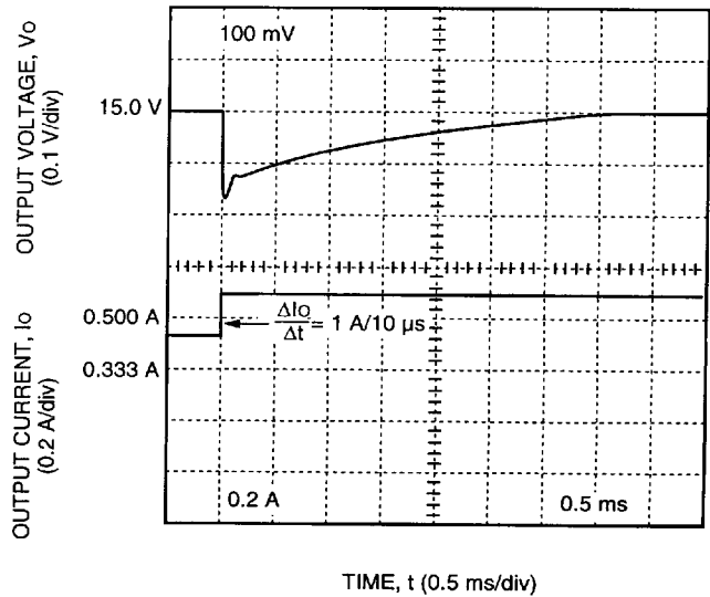
Figure 12. MW010C Typical Output Voltage Waveform for a Step Load Change from 50% to 75% of I_{o,max} ; V_i = 48\text{ V} ; T_A = 25\text{ }^\circ\text{C}
