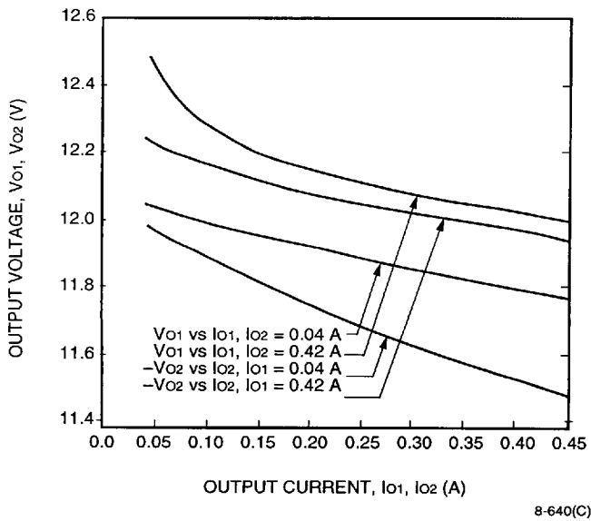
Figure 2. MW010BK Typical Output Voltage Regulation; T_A = 25^\circ\text{C} ; V_i = 48 \text{ V}
