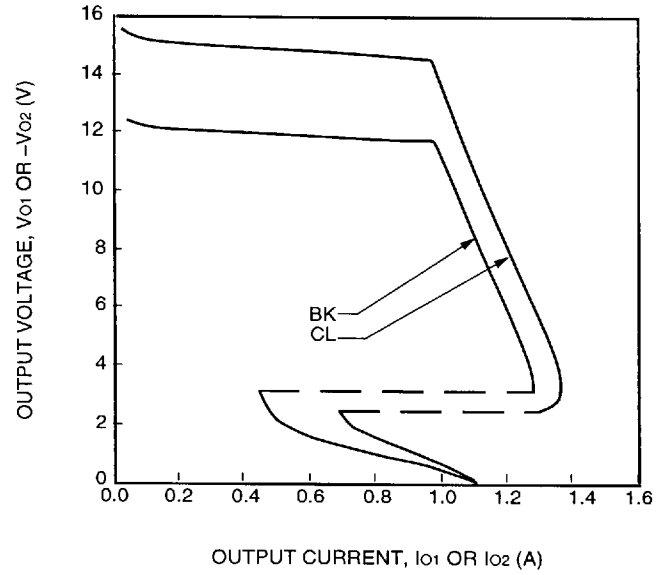
Figure 7. MW010BK, CL Typical Output Characteristic with One Output Fixed at Full Load; V_i = 48\text{ V} ; T_A = 25\text{ }^\circ\text{C}
