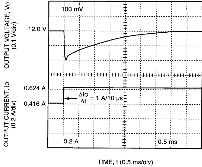
Figure 11. MW010B Typical Output Voltage Waveform for a Step Load Change from 50% to 75% of I_{o,max} ; V_i = 48\text{ V} ; T_A = 25\text{ }^\circ\text{C}
