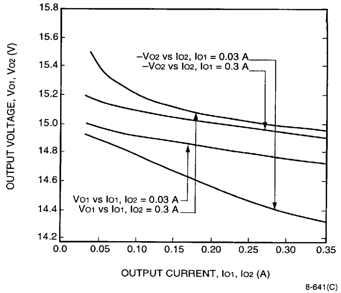
Figure 3. MW010CL Typical Output Voltage Regulation; T_A = 25^\circ\text{C} ; V_i = 48 \text{ V}
