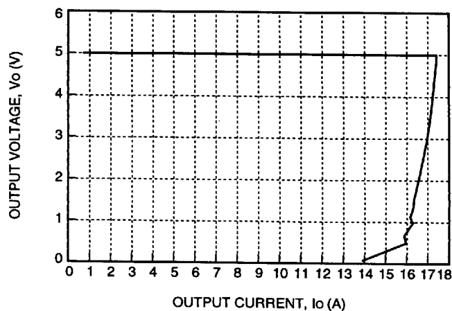
Figure 4. Typical JW075Ax-E Output Characteristics at Room Temperature, V_{IN} = 48 V
