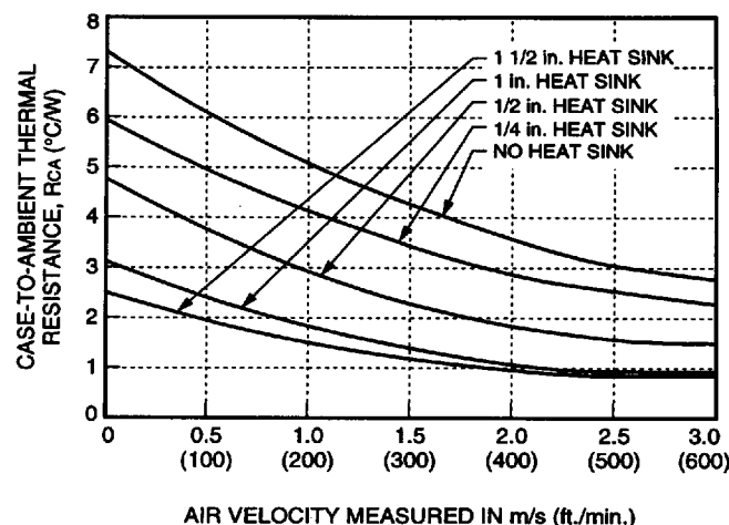
Figure 23. Case-to-Ambient Thermal Resistance Curves; Either Orientation
