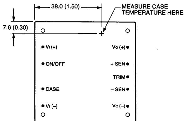
Figure 19. Case Temperature Measurement Location
