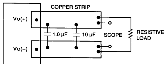
Figure 10. Input Reflected-Ripple Test Setup
