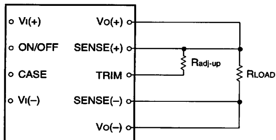
Figure 17. Circuit Configuration to Increase Output Voltage
