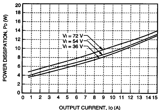
Figure 22. JW075Ax-E Power Dissipation vs. Output Current
