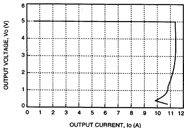
Figure 3. Typical JW050Ax-E Output Characteristics at Room Temperature, V_{IN} = 48 V
