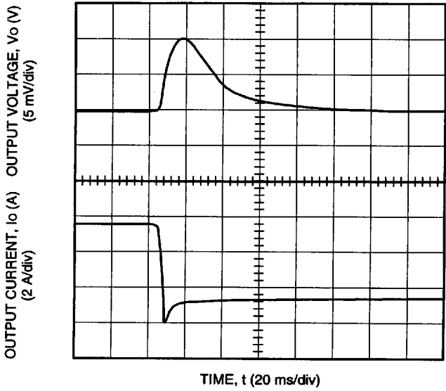
Figure 7. Typical JW075Ax-E Transient Response to Step Decrease in Load from 50% to 25% of Full Load at Room Temperature and 48 V Input (Waveform Averaged to Eliminate Ripple Component.)
