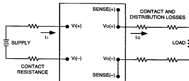
Figure 11. Peak-to-Peak Output Noise Measurement Test Setup
