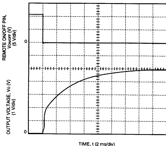
Figure 9. Typical Start-Up from Remote On/Off JW075A1-E; Io = Full Load
