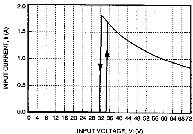
Figure 1. Typical JW050Ax-E Input Characteristics at Room Temperature, I_o = 10 A
