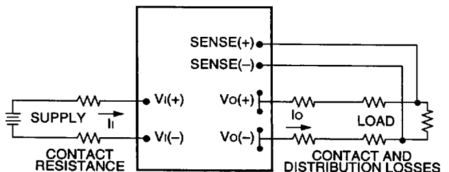
Figure 14. Effective Circuit Configuration for Single-Module Remote-Sense Operation
