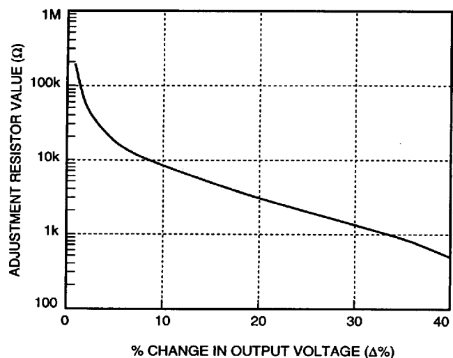
Figure 16. Resistor Selection for Decreased Output Voltage
