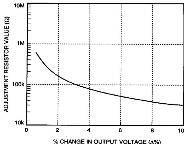
Figure 18. Resistor Selection for Increased Output Voltage
