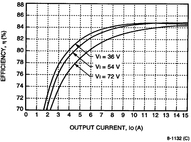
Figure 6. Typical JW075Ax-E Converter Efficiency vs. Output Current at Room Temperature
