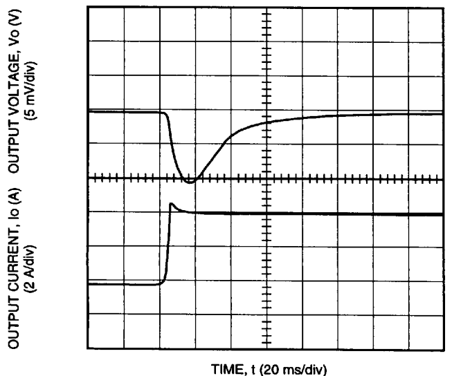
Figure 8. Typical JW075Ax-E Transient Response to Step Increase in Load from 50% to 75% of Full Load at Room Temperature and 48 V Input (Waveform Averaged to Eliminate Ripple Component.)
