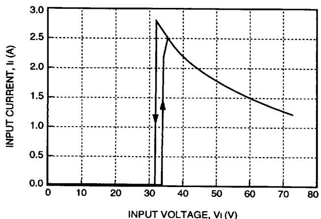
Figure 2. Typical JW075Ax-E Input Characteristics at Room Temperature, I_o = 15 A
