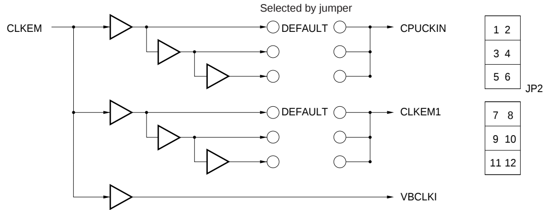
Figure 4-4. Delay Circuit Diagram (IE-V850E-MC-A)
