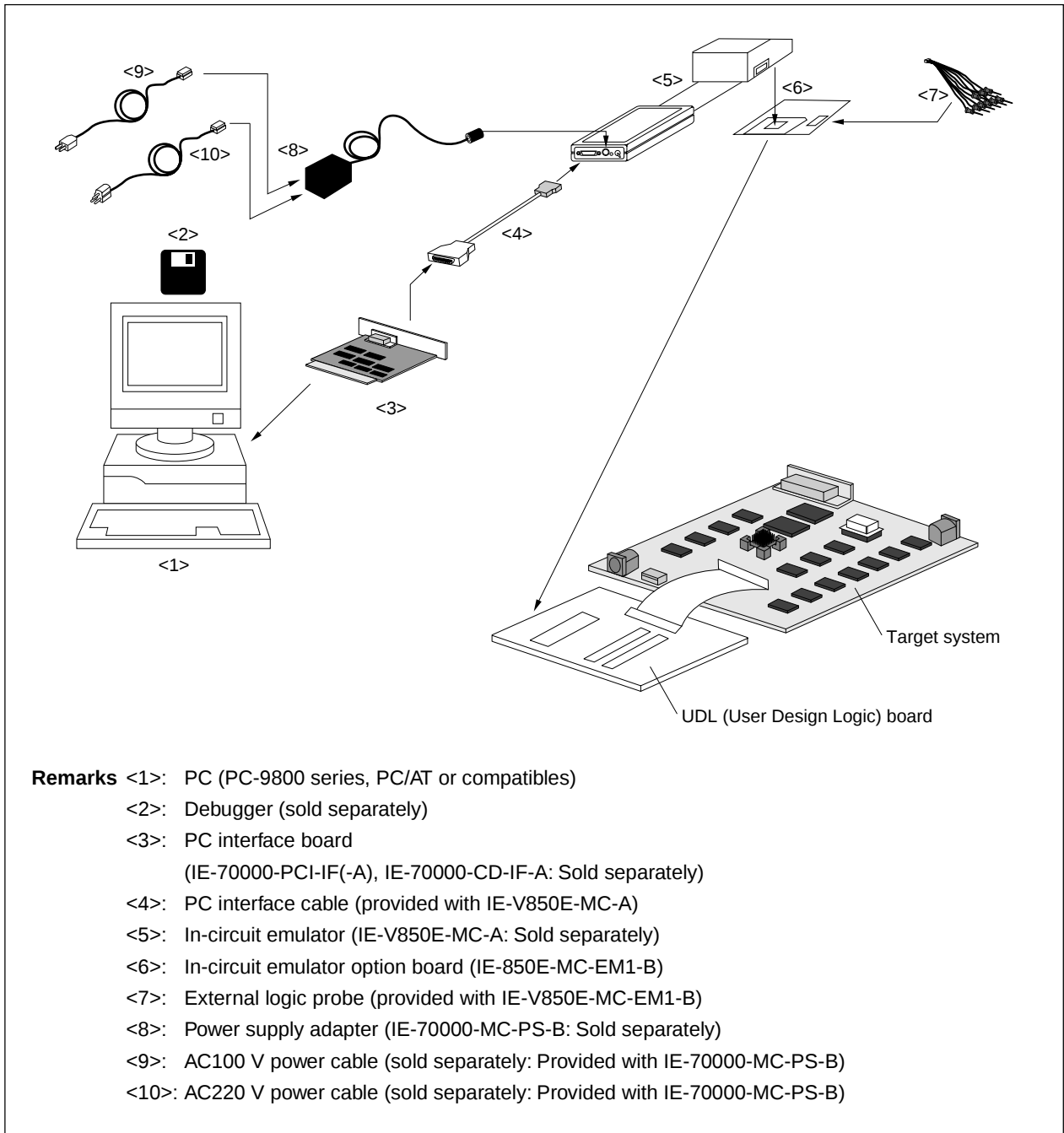
Figure 1-1. System Configuration
