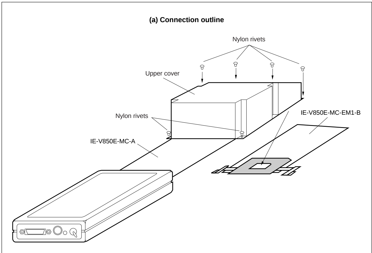
Figure 1-3. Connection of IE-V850E-MC-A and IE-V850E-MC-EM1-B (1/2)
