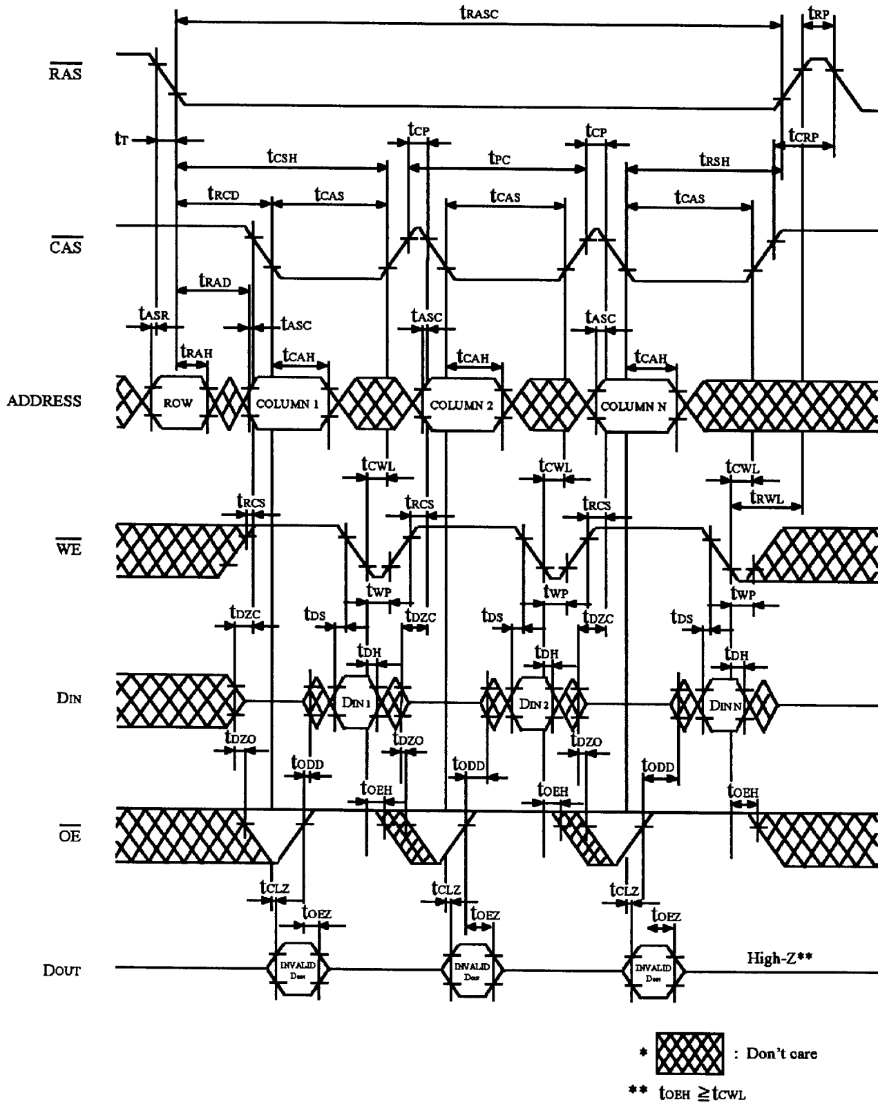
FIGURE 10. FAST PAGE MODE DELAYED WRITE CYCLE
