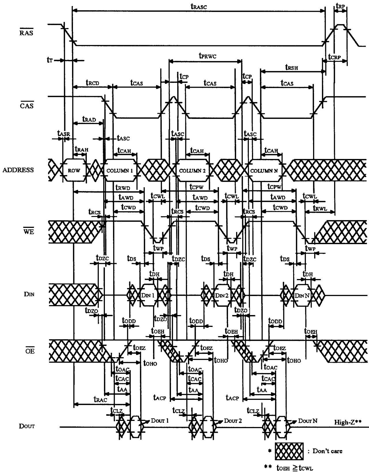
FIGURE 11. FAST PAGE MODE READ MODIFY WRITE CYCLE
