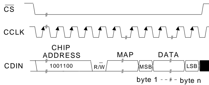
Figure 10. Control Port Timing, SPI mode
