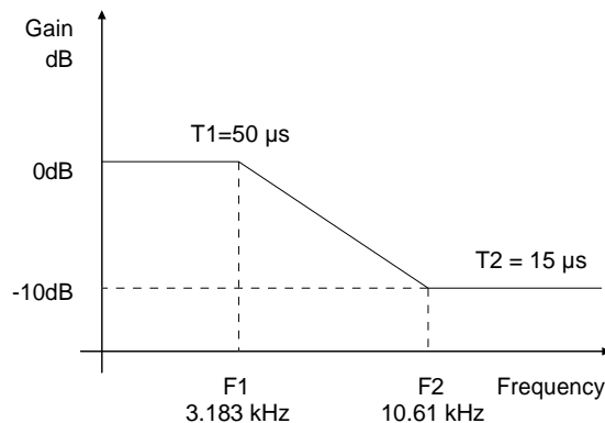
Figure 8. De-Emphasis Curve
