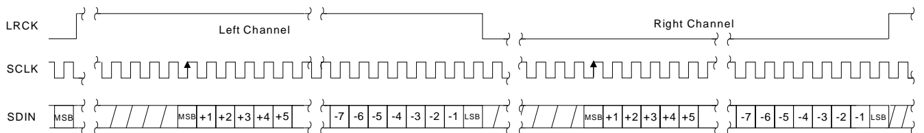
Figure 7. Right-Justified Data
