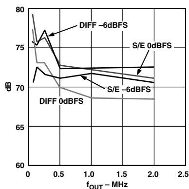
Figure 16. "Out-of-Band" SFDR vs. f_{\text{OUT}} ( f_{\text{DATA}}/2 to 3/2 f_{\text{DATA}} )
