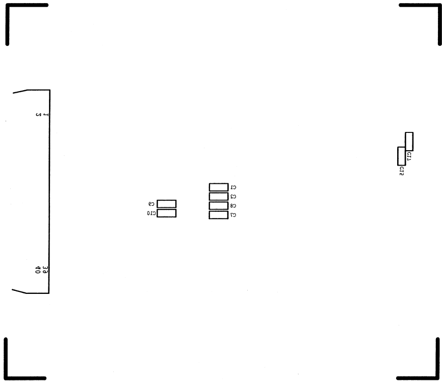
Figure 48. Silkscreen Layer—Bottom
