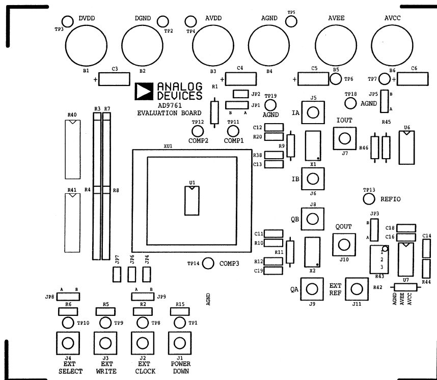
Figure 43. Silkscreen Layer—Top
