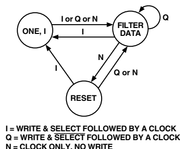
Figure 29. State Transition Diagram of AD9761 Digital Interface
