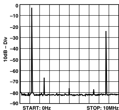
Figure 13. Single-Tone SFDR (DC to 2 f_{\text{DATA}} , f_{\text{CLOCK}} = 2 f_{\text{DATA}} )
