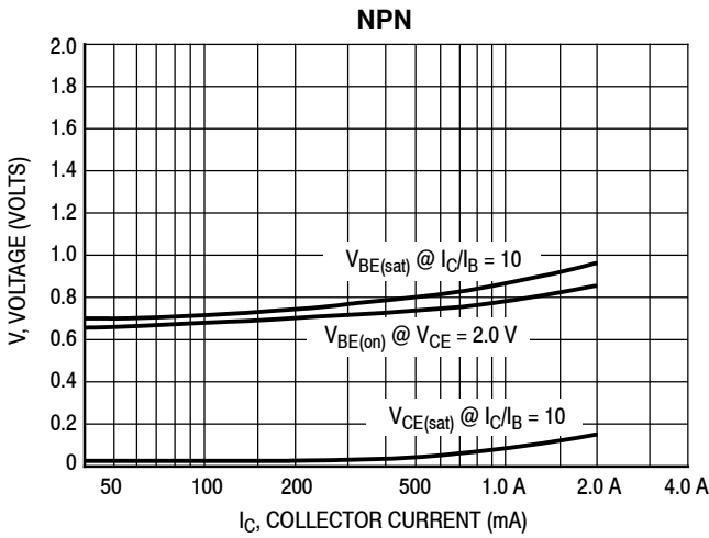
Figure 3. On Voltages
