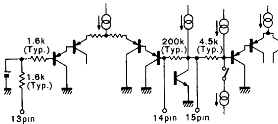
Figure 13 FG control amplifier (pins 13 ~ 15)
