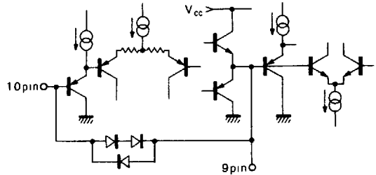
Figure 10 Error amplifier (pins 9, 10)
