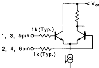
Figure 9 Hall inputs (pins 1 ~ 6)
