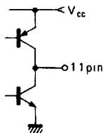
Figure 11 Speed discriminator (pin 11)
