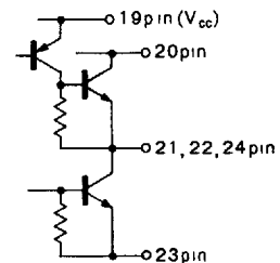
Figure 16 Motor output (pins 19 ~ 24)
