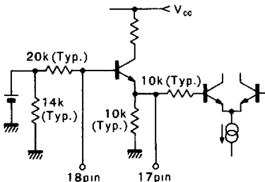
Figure 15 Oscillator (pins 17 and 18)
