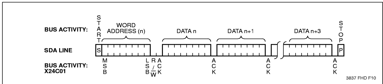
Figure 5. Page Write
