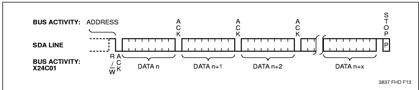
Figure 8. Sequential Read
