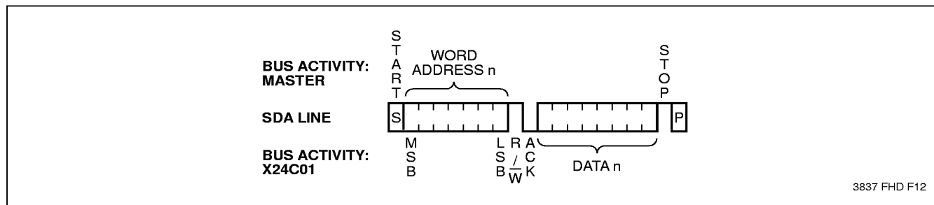
Figure 7. Byte Read
