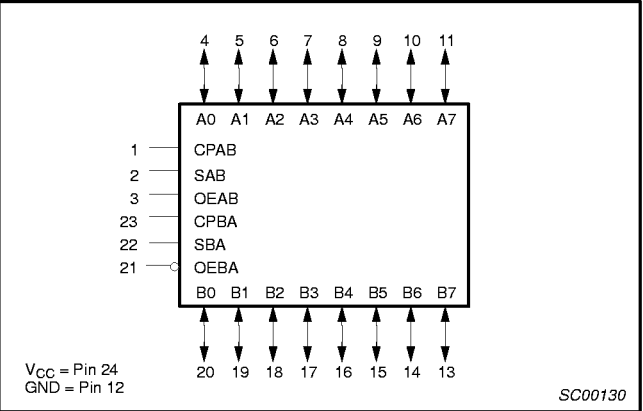
LOGIC SYMBOL – 74ALS652/652-1
