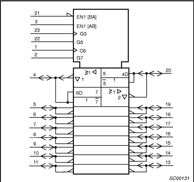
IEC/IEEE SYMBOL – 74ALS651/651-1
