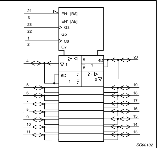
IEC/IEEE SYMBOL – 74ALS652/652-1
