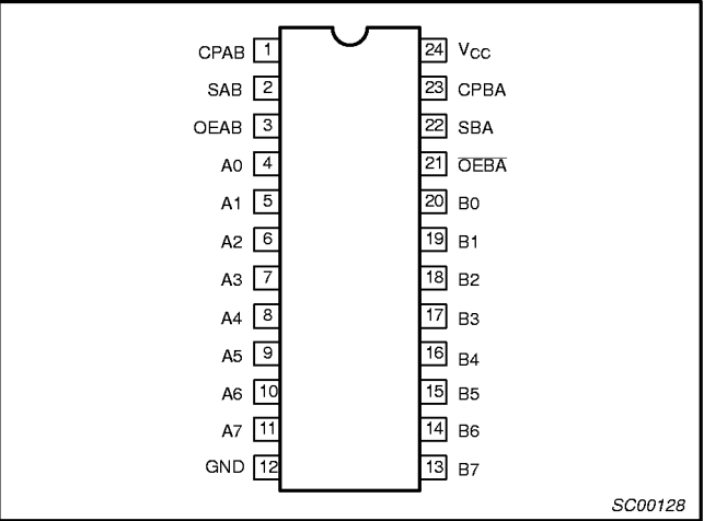
PIN CONFIGURATION – 74ALS652/652-1
