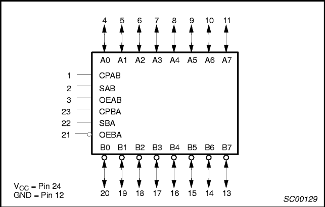
LOGIC SYMBOL – 74ALS651/651-1
