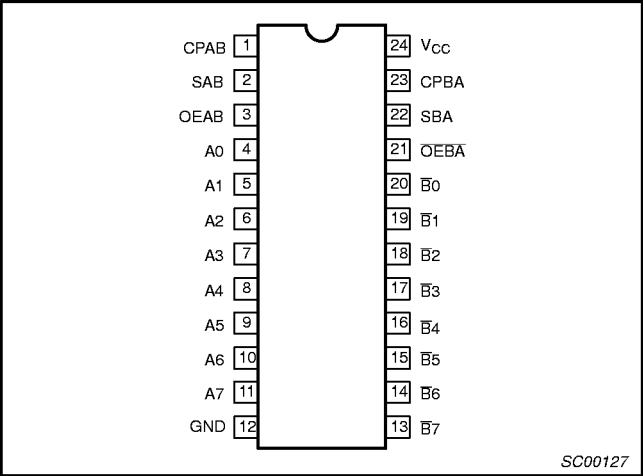
PIN CONFIGURATION – 74ALS651/651-1
