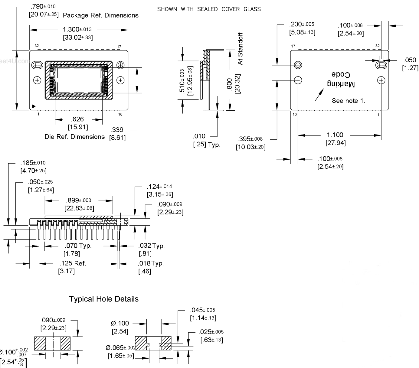
Figure 15: Completed Assembly (1 of 2)
