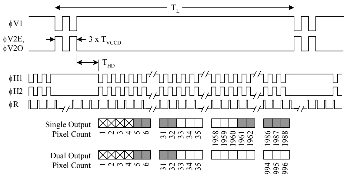
Figure 13: Line Timing
