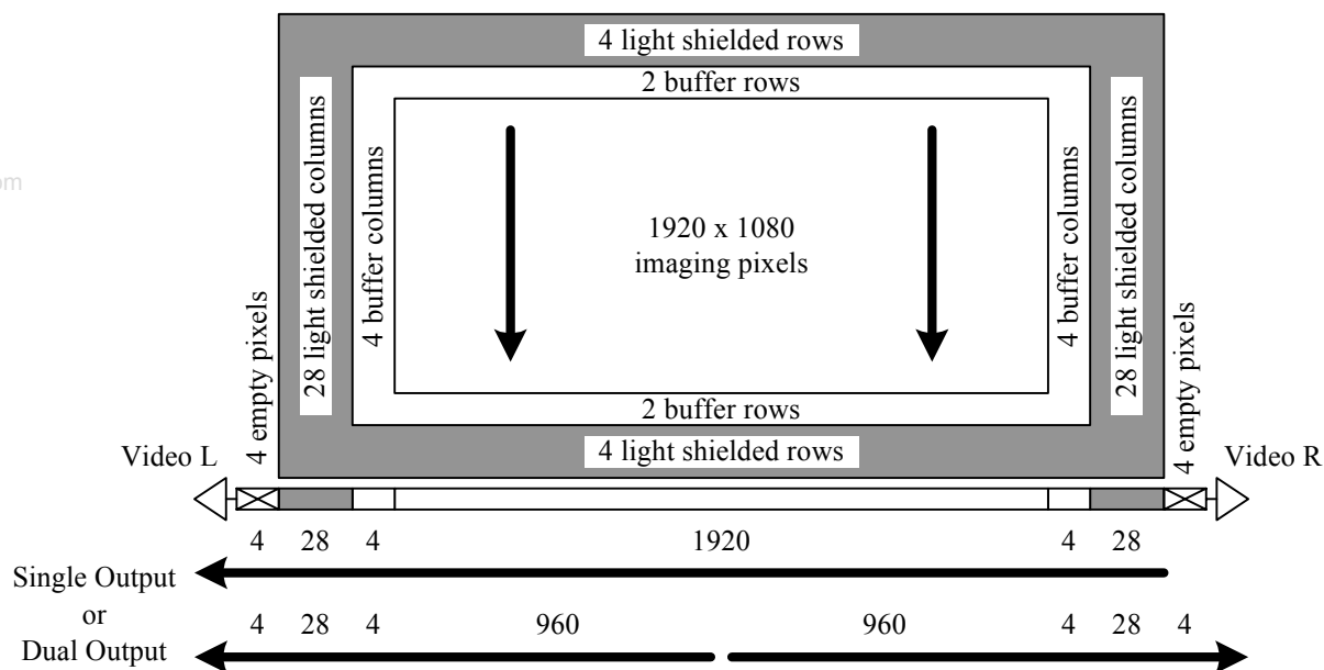
Figure 1: Sensor Architecture
