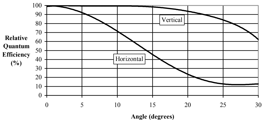
Figure 4: Angular Dependence of Quantum Efficiency
