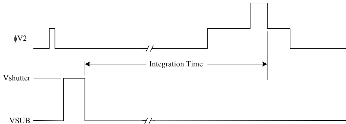
Figure 14: Electronic Shutter Timing Diagram
