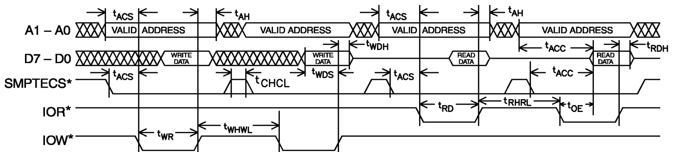
FIGURE 3 — Host Processor Bus Timing
