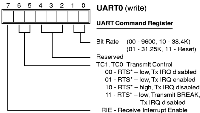
UART Command/Status Register
