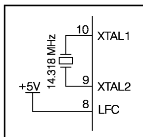
Fig. 4 - Crystal Oscillator
