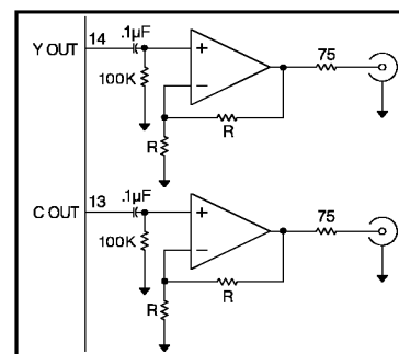
Fig. 7 - Video Output
