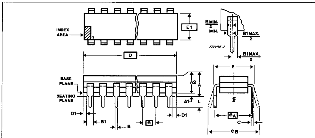
28 PINS CERDIP .300
