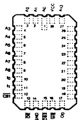
Pinout LCC 28 pins (top view)
