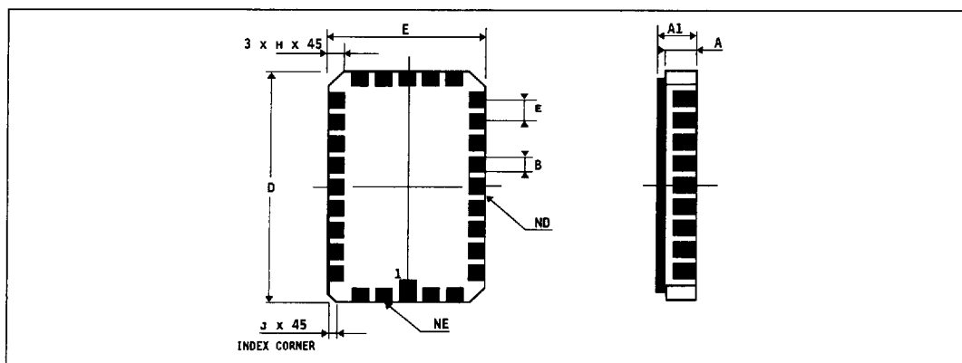
28 LDS .050 CENTER LEADLESS RECTANGULAR CHIP CARRIER
