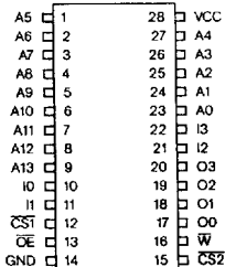
Pinout DIL 28 pins (top view)
