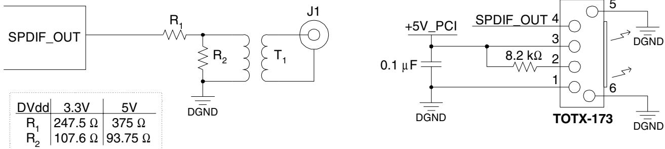
Figure 15. S/PDIF Output
