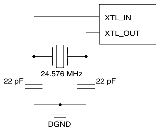
Figure 17. External Crystal
