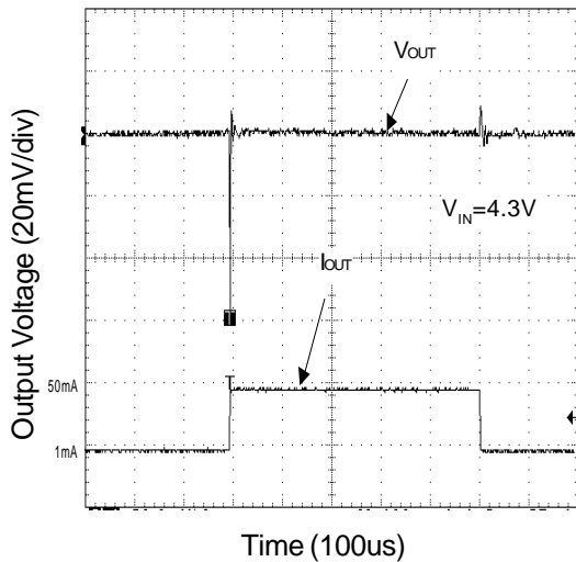
Load-Transient Response
