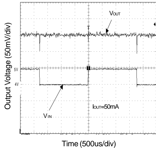
Line-Transient Response
