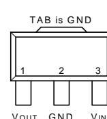
SOT-89 (Top View)
