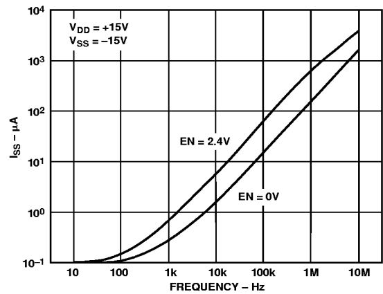
Figure 12. Negative Supply Current vs. Switching Frequency
