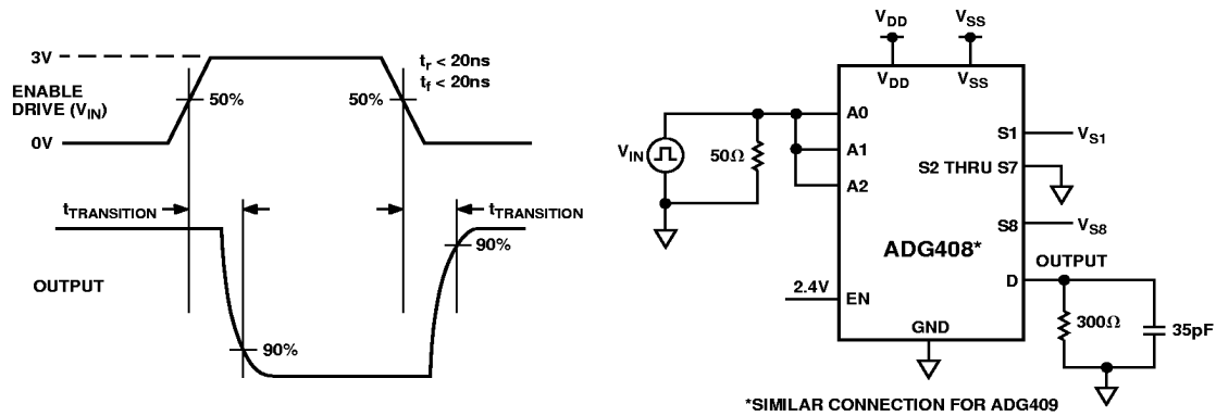
Test Circuit 5. Switching Time of Multiplexer, t_{TRANSITION}
