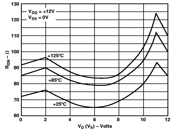
Figure 5. R_{ON} as a Function of V_D ( V_S ) for Different Temperatures
