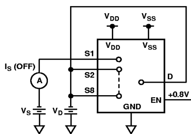
Test Circuit 2. I_S (OFF)
