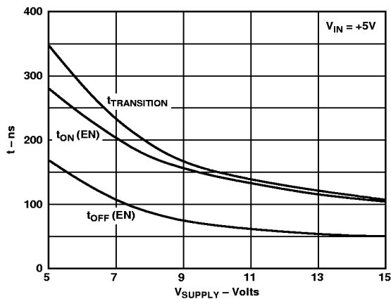
Figure 8. Switching Time vs. Single Supply
