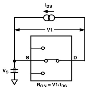
Test Circuit 1. On Resistance
