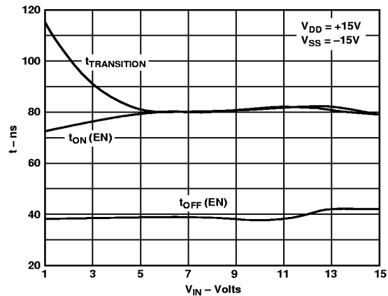
Figure 7. Switching Time vs. V_{IN} (Bipolar Supply)
