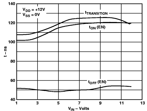
Figure 10. Switching Time vs. V_{IN} (Single Supply)
