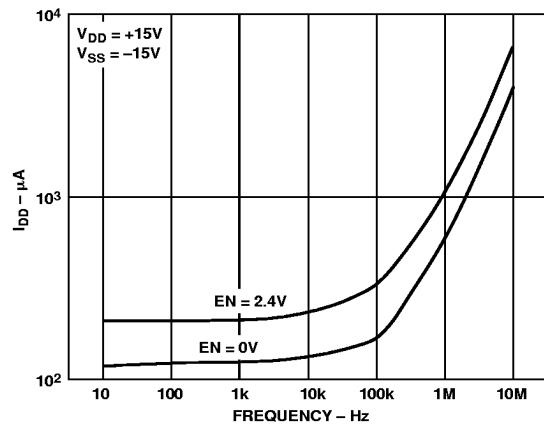
Figure 9. Positive Supply Current vs. Switching Frequency
