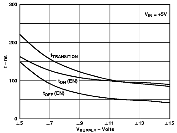
Figure 11. Switching Time vs. Bipolar Supply
