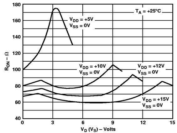
Figure 4. R_{ON} as a Function of V_D ( V_S ): Single Supply Voltage
