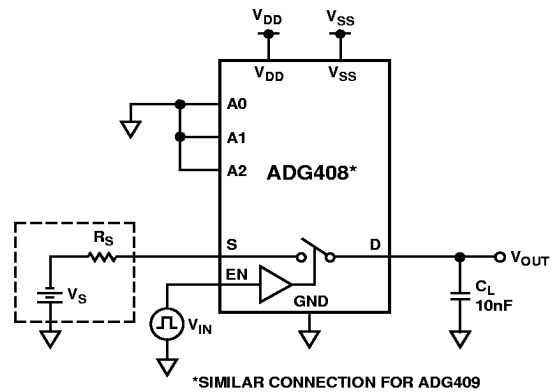
Test Circuit 8. Charge Injection
