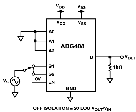
Test Circuit 9. OFF Isolation
