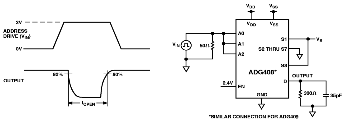
Test Circuit 6. Break-Before-Make Delay, t_{OPEN}
