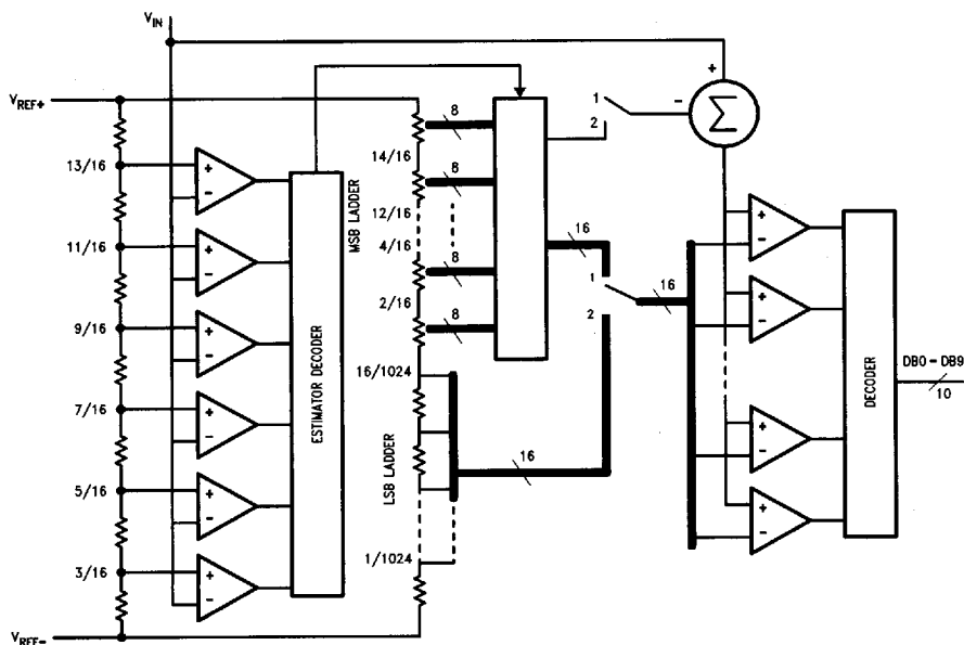
FIGURE 3. Block Diagram of the Multistep Converter Architecture
