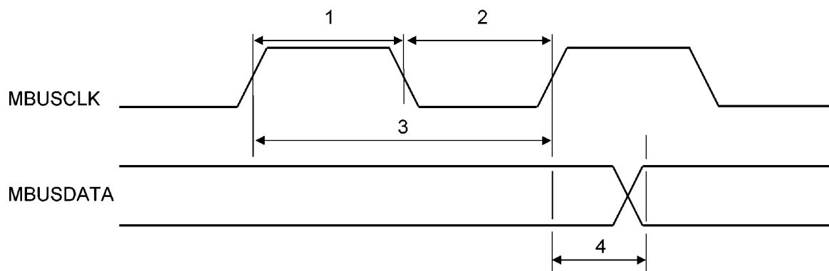
Magic Bus Output and Clock Timing (Master, PHAPOL=1)
