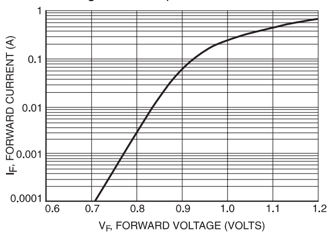
Figure 3. Forward Voltage
