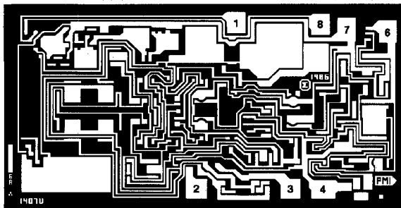
DIE SIZE 0.100 × 0.055 inch, 5500 sq. mils (2.54 × 1.40 mm, 3.56 sq. mm)
