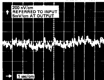
OP-07 LOW FREQUENCY NOISE
