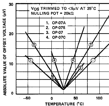
TRIMMED OFFSET VOLTAGE vs TEMPERATURE
