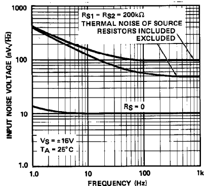
TOTAL INPUT NOISE VOLTAGE vs FREQUENCY
