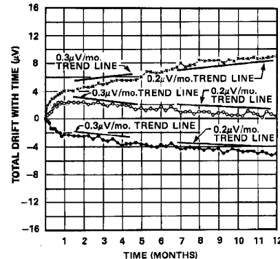
OFFSET VOLTAGE STABILITY vs TIME
