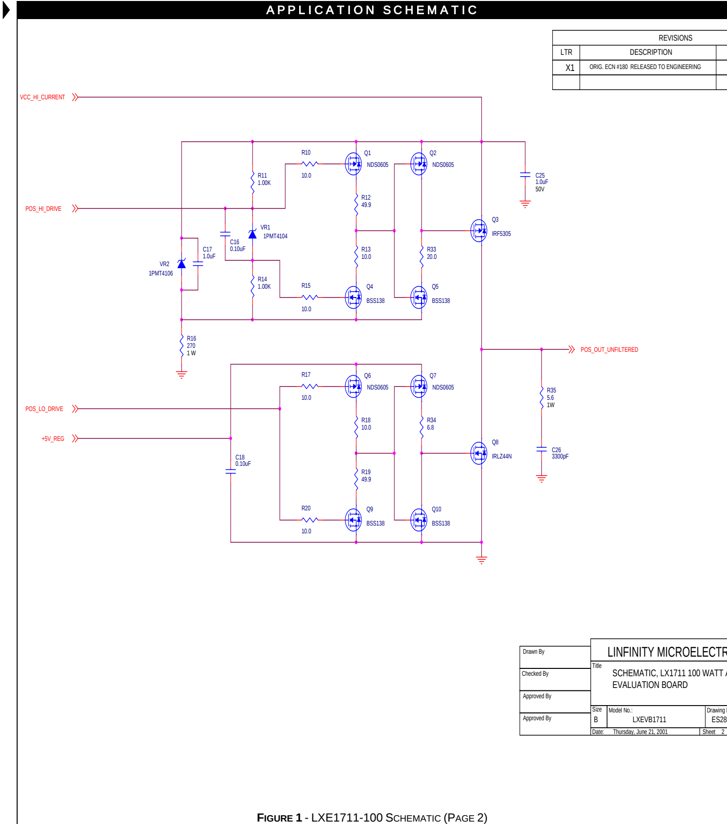
FIGURE 1 - LX1711-100 SCHEMATIC (PAGE 2)
