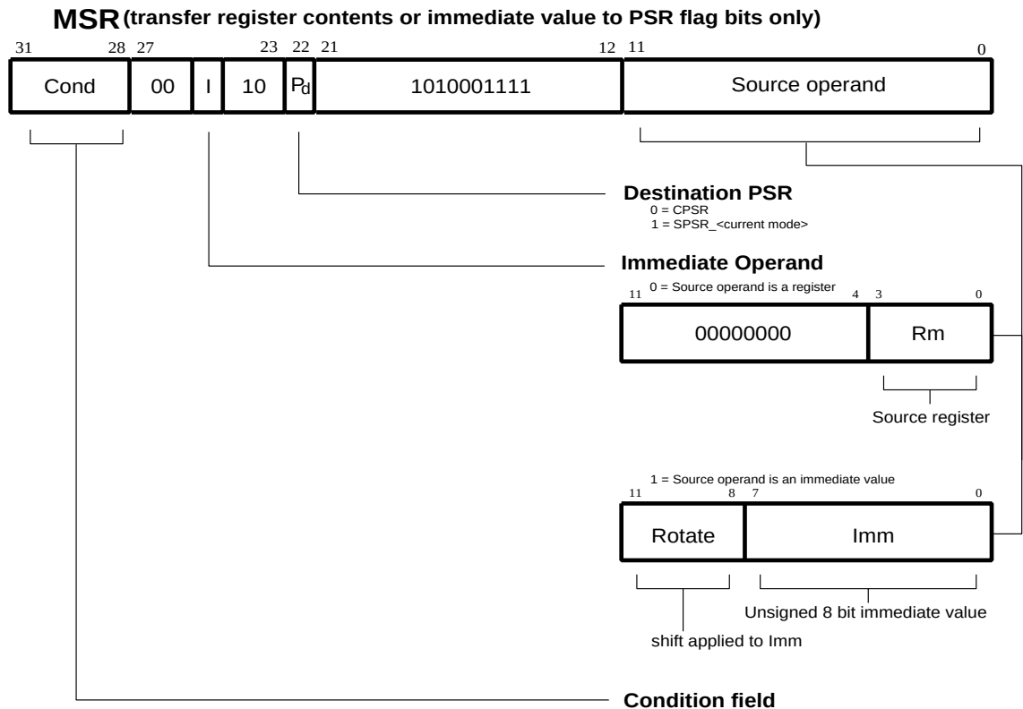
Figure 15: PSR Transfer
