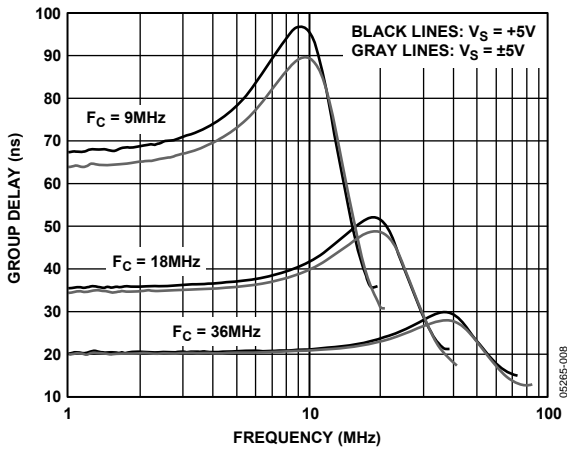
Figure 10. Group Delay vs. Frequency, Power Supply, and Cutoff Frequency
