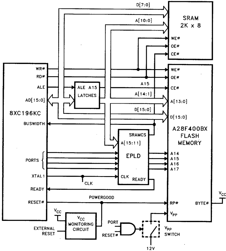
Figure 1. A28F400BX Interface to 8XC196KC
