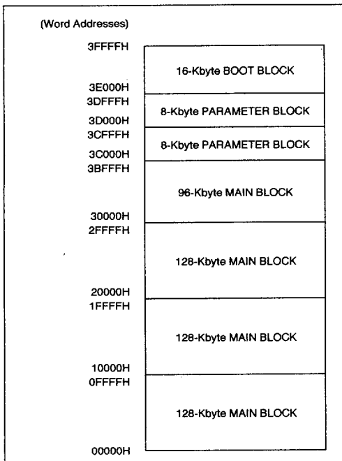
Figure 5. A28F400BX-T Memory Map
