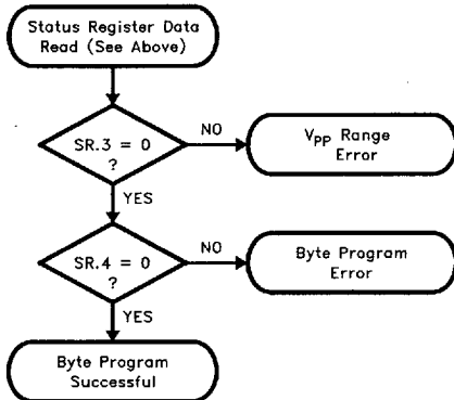
Figure 6. Automated Byte Programming Flowchart
