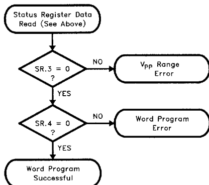
Figure 7. Automated Word Programming Flowchart
