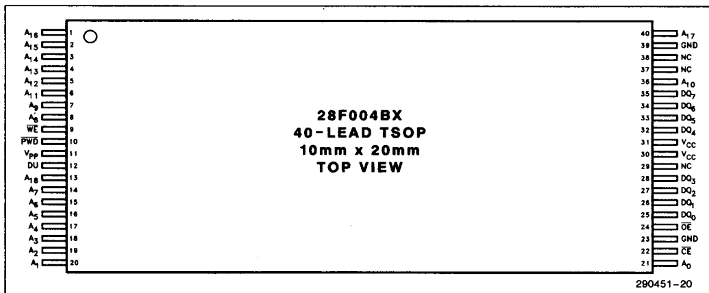
Figure 5. TSOP Lead Configuration for x8 28F004BX
