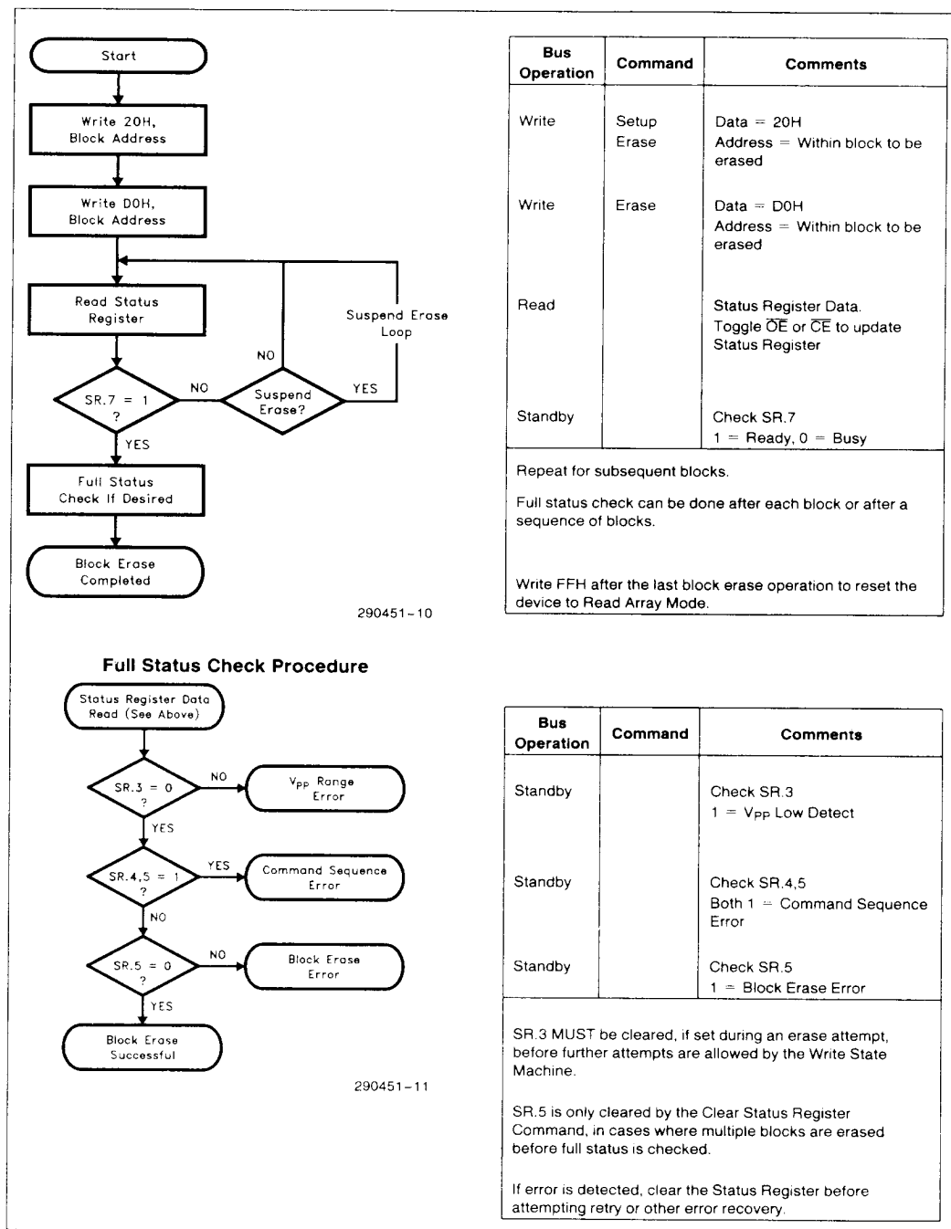
Figure 14. Automated Block Erase Flowchart
