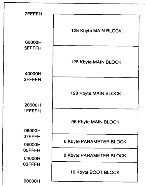
Figure 10. 28F004BX-B Memory Map
