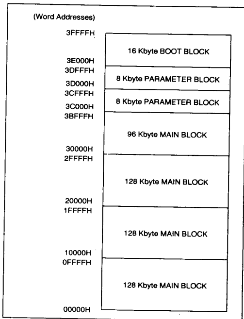
Figure 8. 28F400BX-T Memory Map
