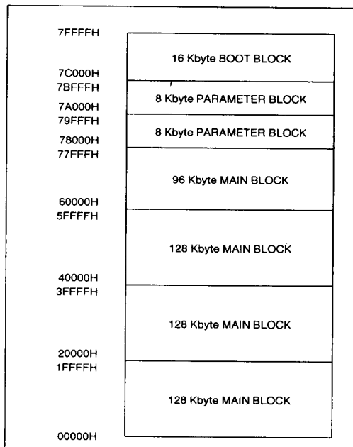
Figure 11. 28F004BX-T Memory Map
