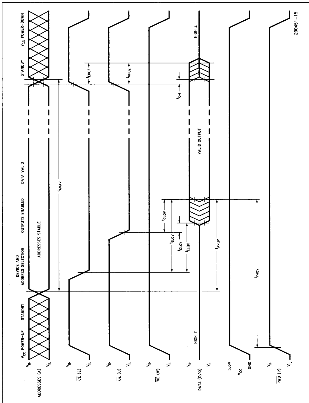
Figure 16. A.C. Waveforms for Read Operations
