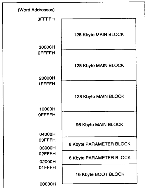
Figure 7. 28F400BX-B Memory Map
