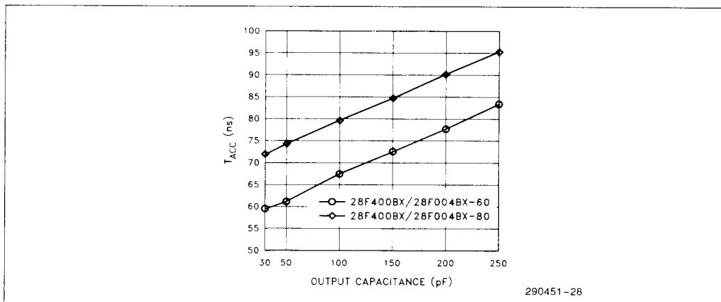
Figure 19. T ACC vs Output Load Capacitance
