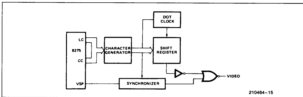
Figure 15. Typical Dot Level Block Diagram
