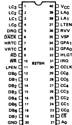
210464-2 Figure 2. Pin Configuration
