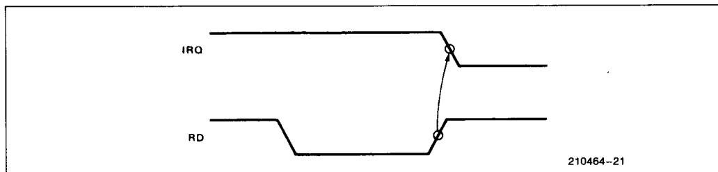
Figure 21. End of Interrupt Request
