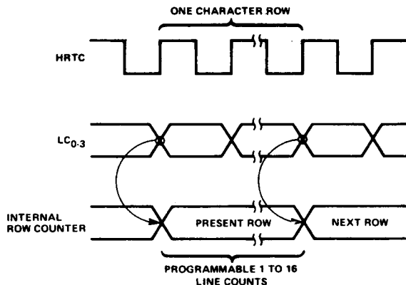
Figure 17. Row Timing
