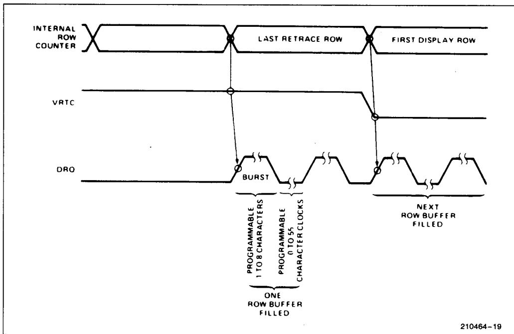
Figure 19. DMA Timing
