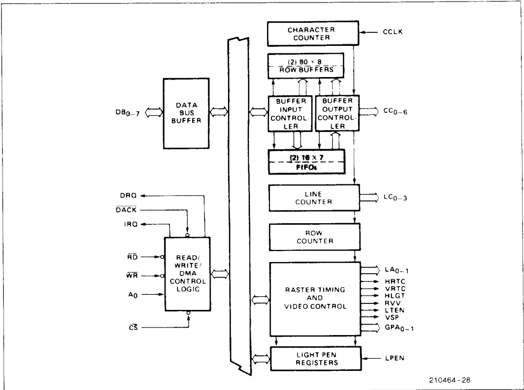
Figure 24. Block Diagram Showing FIFO Activation
