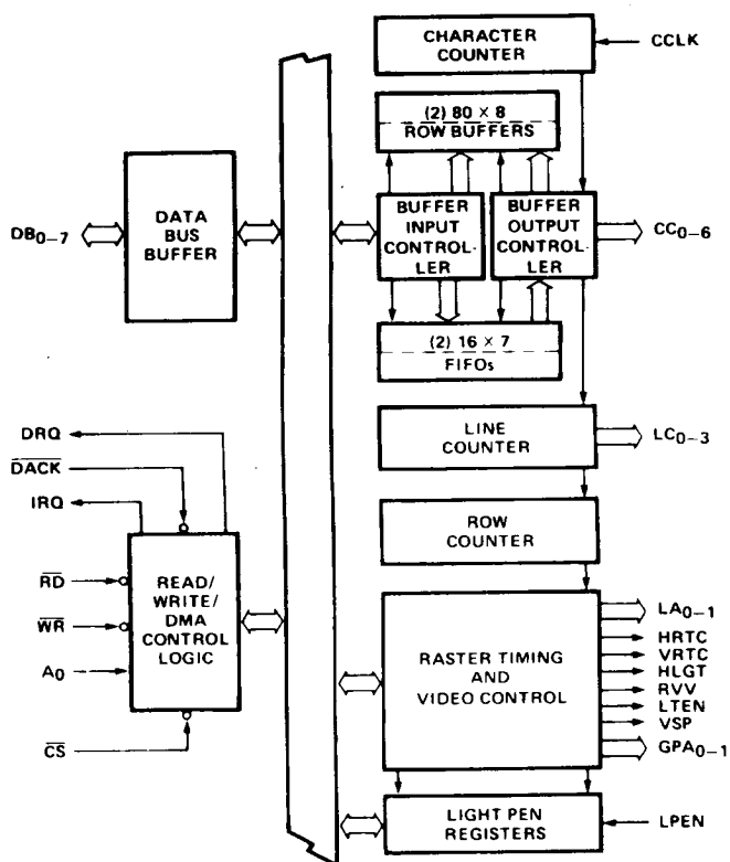
Figure 1. Block Diagram
