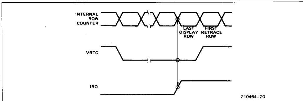
Figure 20. Beginning of Interrupt Request
