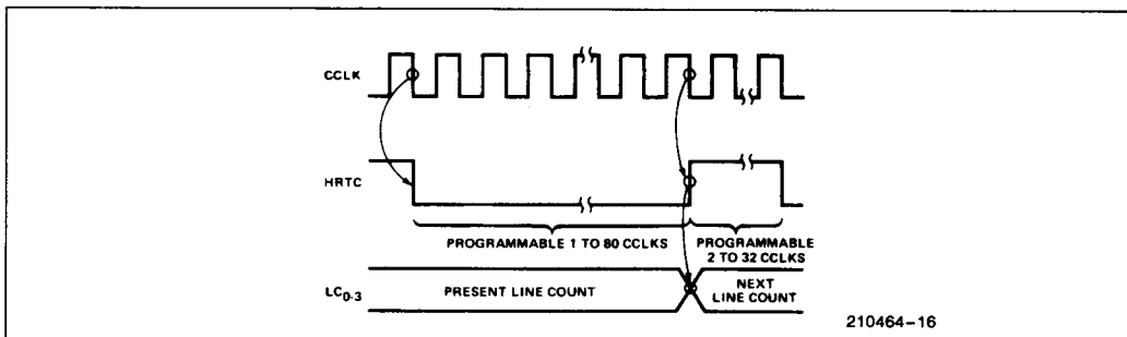
Figure 16. Line Timing
