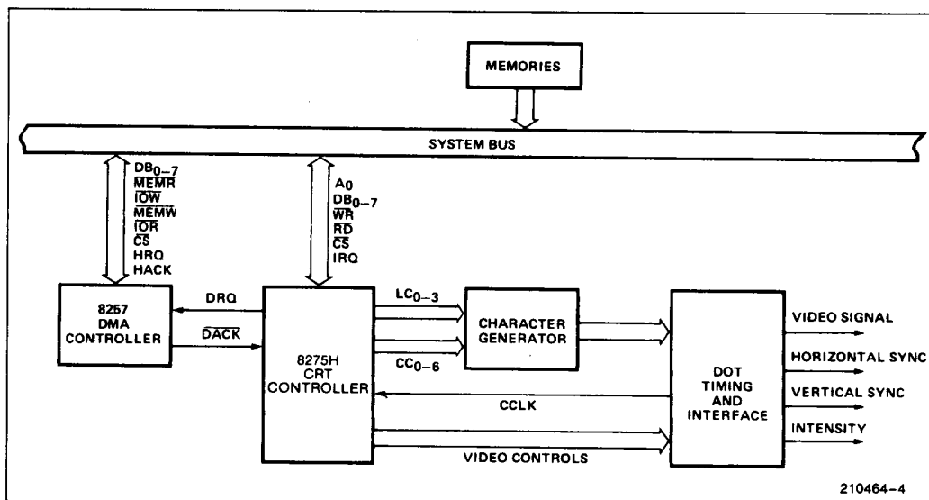
Figure 4. 8275H Systems Block Diagram Showing Systems Operation
