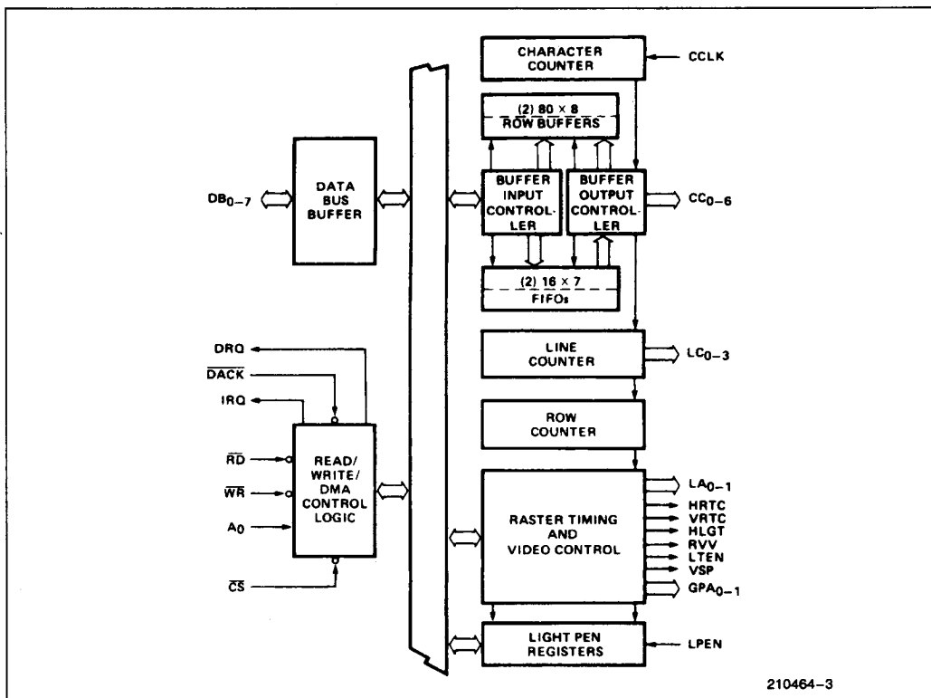
Figure 3. 8275H Block Diagram Showing Counter and Register Functions
