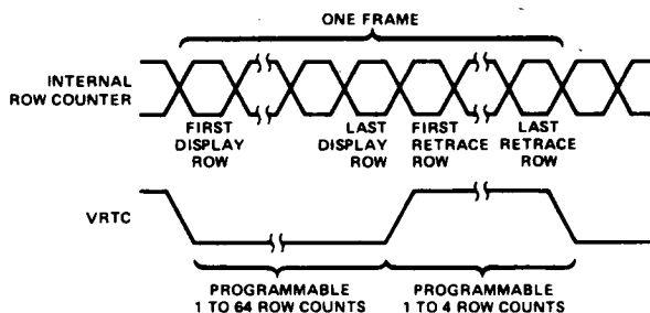
Figure 18. Frame Timing
