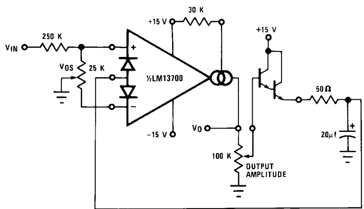
FIGURE 7. AGC Amplifier
