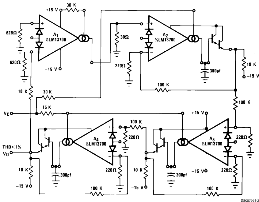
FIGURE 17. Sinusoidal VCO
