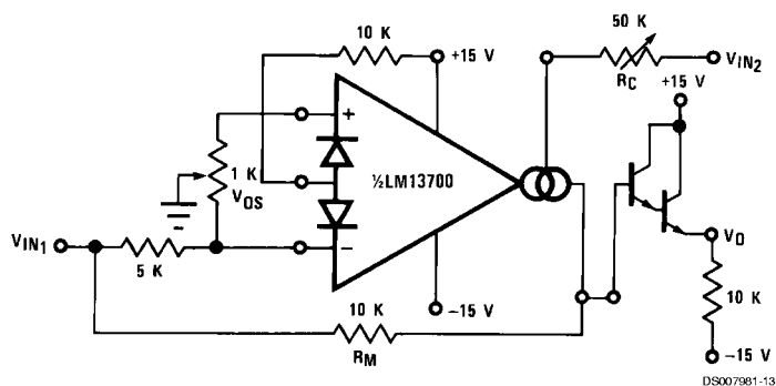
FIGURE 6. Four-Quadrant Multiplier
