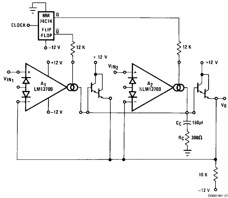
FIGURE 20. Multiplexer
