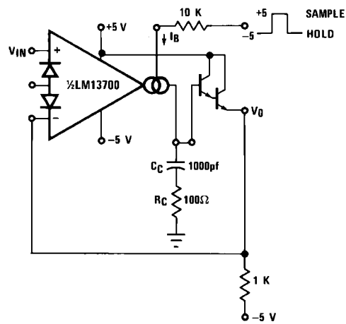
FIGURE 25. Sample-Hold Circuit
