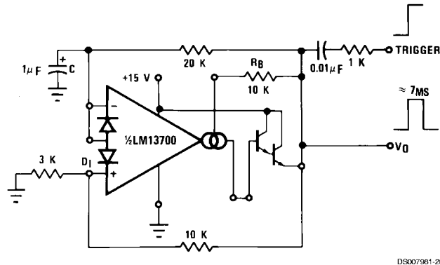
FIGURE 19. Zero Stand-By Power Timer
