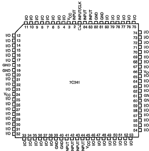
PLCC/HLCC Top View
