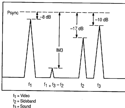
Figure 2. 3-Tone TV Intermodulation Test
