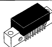
CASE 714P-03, STYLES 2, 3 CA4800C, CA4812C, CA4815C
