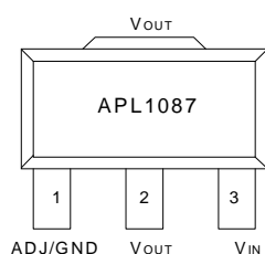
SOT-89 (Front View)
