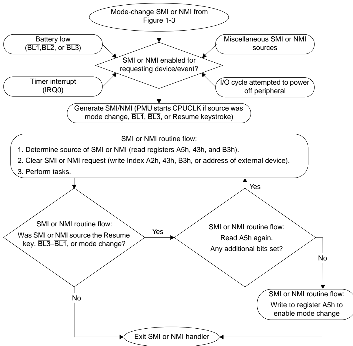
Figure 1-4 SMI Processing Flowchart
