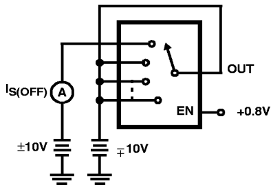
FIGURE 3. I_{S(OFF)} (NOTE 1)
