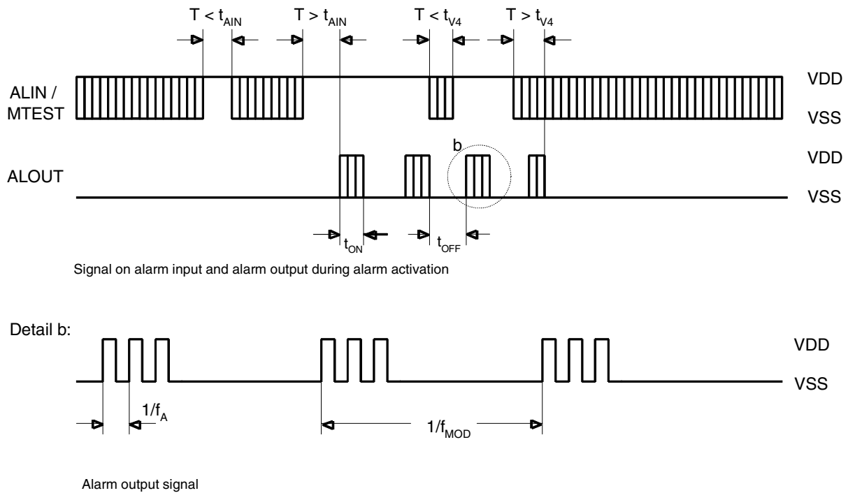
Figure 4. Alarm Operation
