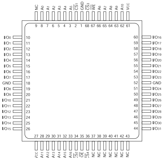
FIG. 3 PIN CONFIGURATION FOR WS128K32-XG2UX, WS128K32-XG2LX, WS128K32-XG1TX AND WS128K32-XG1UX 1
