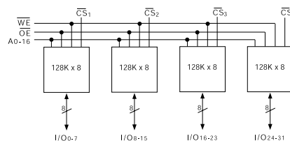
FIG. 3 PIN CONFIGURATION FOR WS128K32-XG2UX, WS128K32-XG2LX, WS128K32-XG1TX AND WS128K32-XG1UX 1
