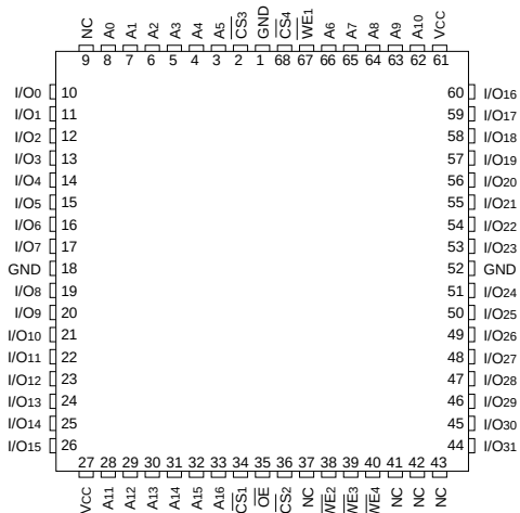
FIG. 3 PIN CONFIGURATION FOR WF128K32-XG1UX5 1 , WF128K32-XG1TX5 AND WF128K32-XG2UX5, WF128K32-XG2LX5
