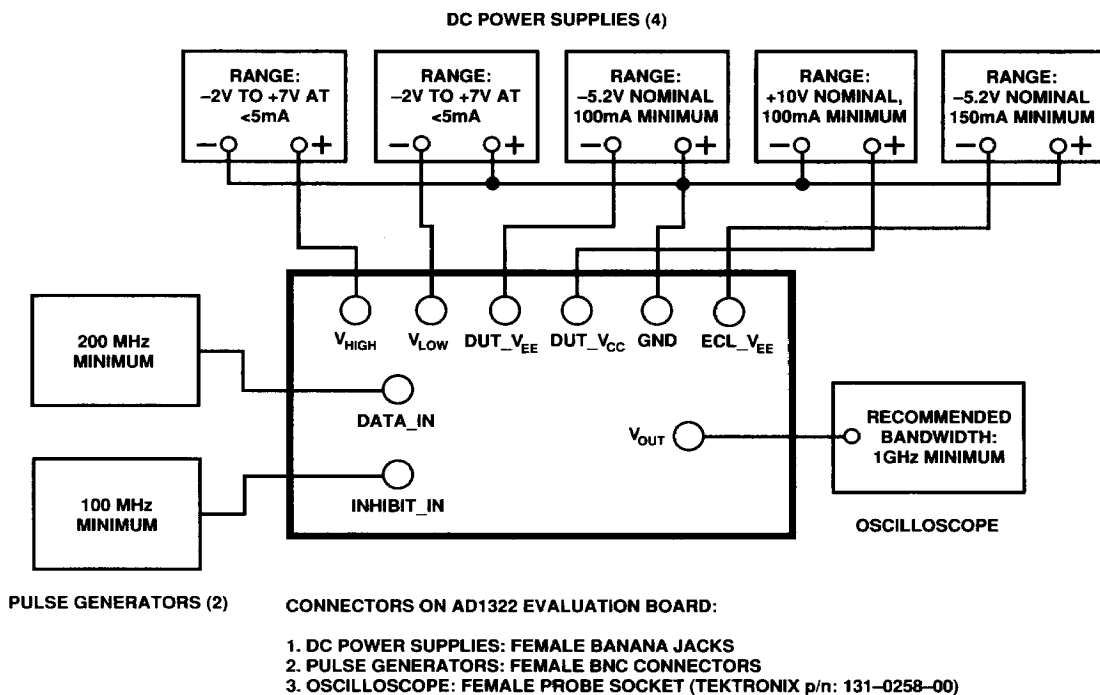
Figure 20. AD1322 Evaluation Board Connections
