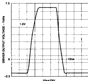
Figure 11. V_{OUT} = 9 V as Seen at the End of a 28", 50 \Omega Cable
