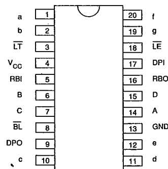
top view 20-pin DIP
